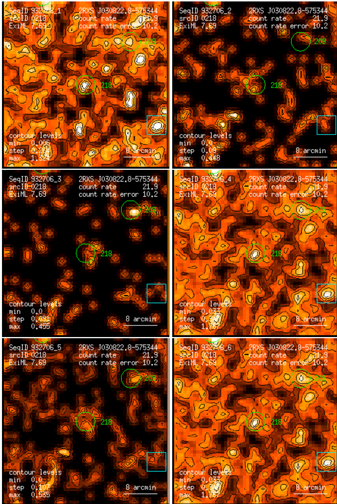
Figure 218: RASS 932706: detection 0218: band rate images, Gaussian filter: (1) PSPC channels 11 – 41, (2) 52 – 90, (3) 91 – 201, (4) 11 – 235, (5) 52 – 201, (6) 11 – 201. Broad band rates in counts/ks. Band rate contour levels in counts/ks/arcmin 2 .
