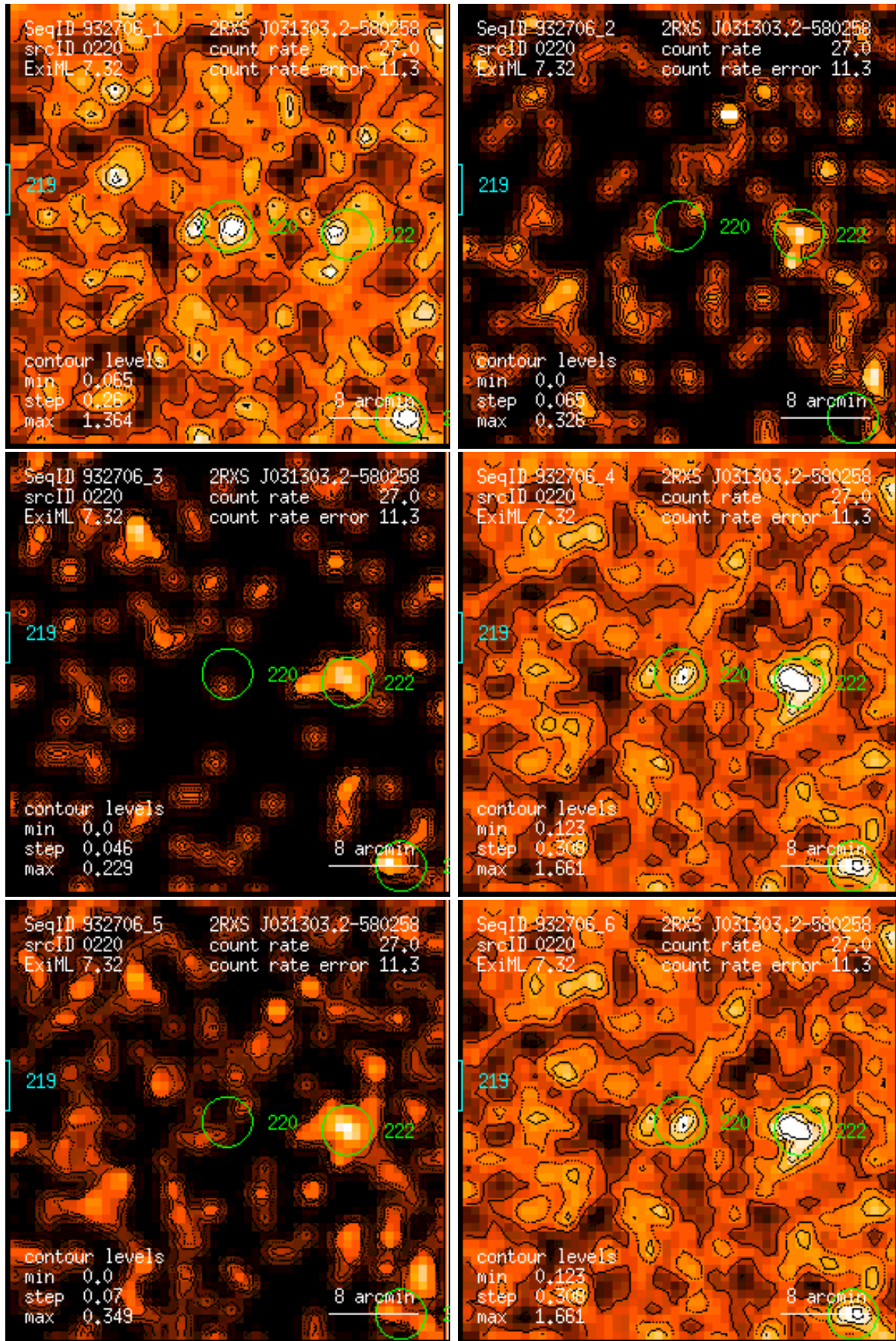
Figure 220: RASS 932706: detection 0220: band rate images, Gaussian filter: (1) PSPC channels 11 – 41, (2) 52 – 90, (3) 91 – 201, (4) 11 – 235, (5) 52 – 201, (6) 11 – 201. Broad band rates in counts/ks. Band rate contour levels in counts/ks/arcmin 2 .
