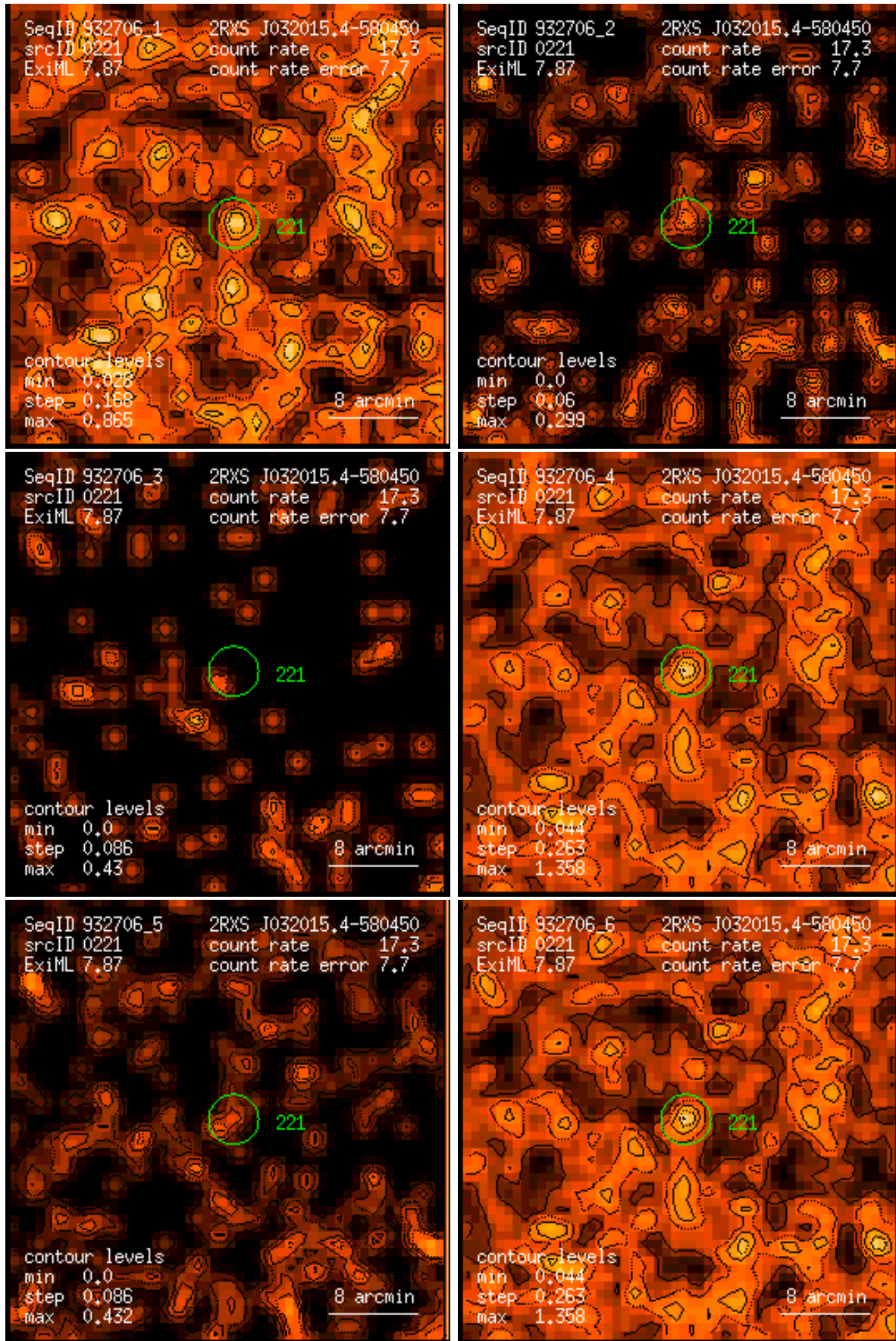
Figure 221: RASS 932706: detection 0221: band rate images, Gaussian filter: (1) PSPC channels 11 – 41, (2) 52 – 90, (3) 91 – 201, (4) 11 – 235, (5) 52 – 201, (6) 11 – 201. Broad band rates in counts/ks. Band rate contour levels in counts/ks/arcmin 2 .
