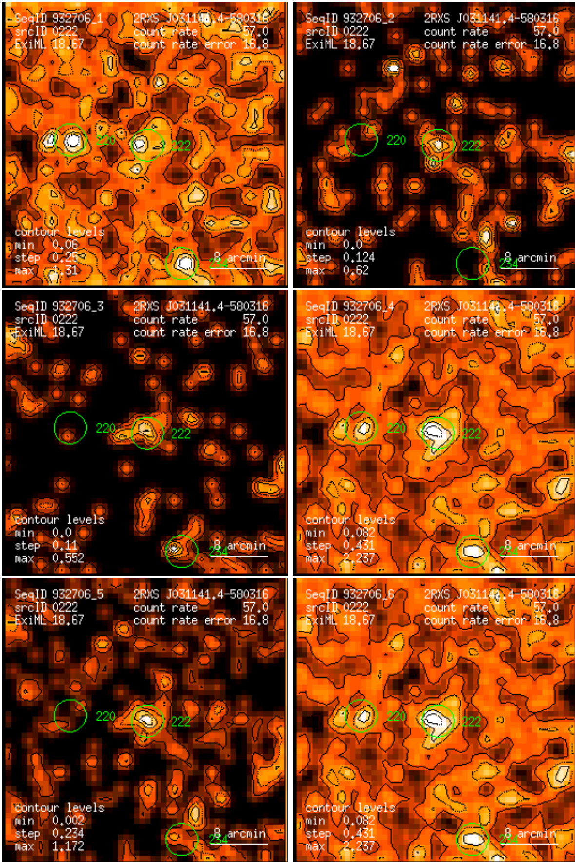
Figure 222: RASS 932706: detection 0222: band rate images, Gaussian filter: (1) PSPC channels 11 – 41, (2) 52 – 90, (3) 91 – 201, (4) 11 – 235, (5) 52 – 201, (6) 11 – 201. Broad band rates in counts/ks. Band rate contour levels in counts/ks/arcmin 2 .
