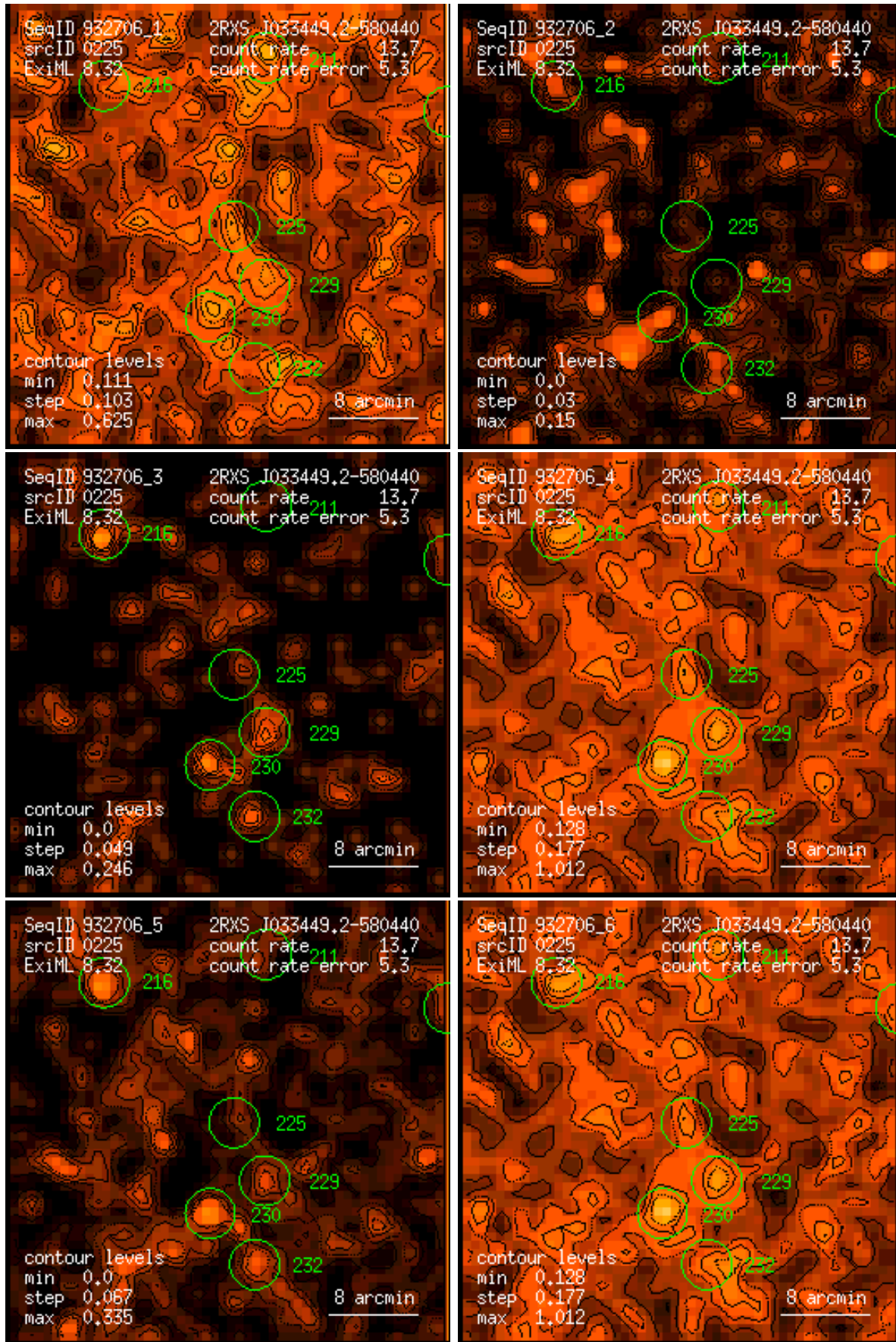
Figure 225: RASS 932706: detection 0225: band rate images, Gaussian filter: (1) PSPC channels 11 – 41, (2) 52 – 90, (3) 91 – 201, (4) 11 – 235, (5) 52 – 201, (6) 11 – 201. Broad band rates in counts/ks. Band rate contour levels in counts/ks/arcmin 2 .
