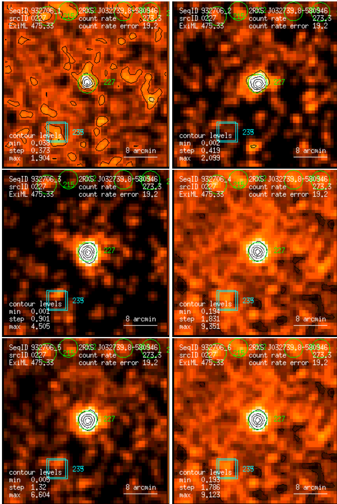
Figure 227: RASS 932706: detection 0227: band rate images, Gaussian filter: (1) PSPC channels 11 – 41, (2) 52 – 90, (3) 91 – 201, (4) 11 – 235, (5) 52 – 201, (6) 11 – 201. Broad band rates in counts/ks. Band rate contour levels in counts/ks/arcmin 2 .
