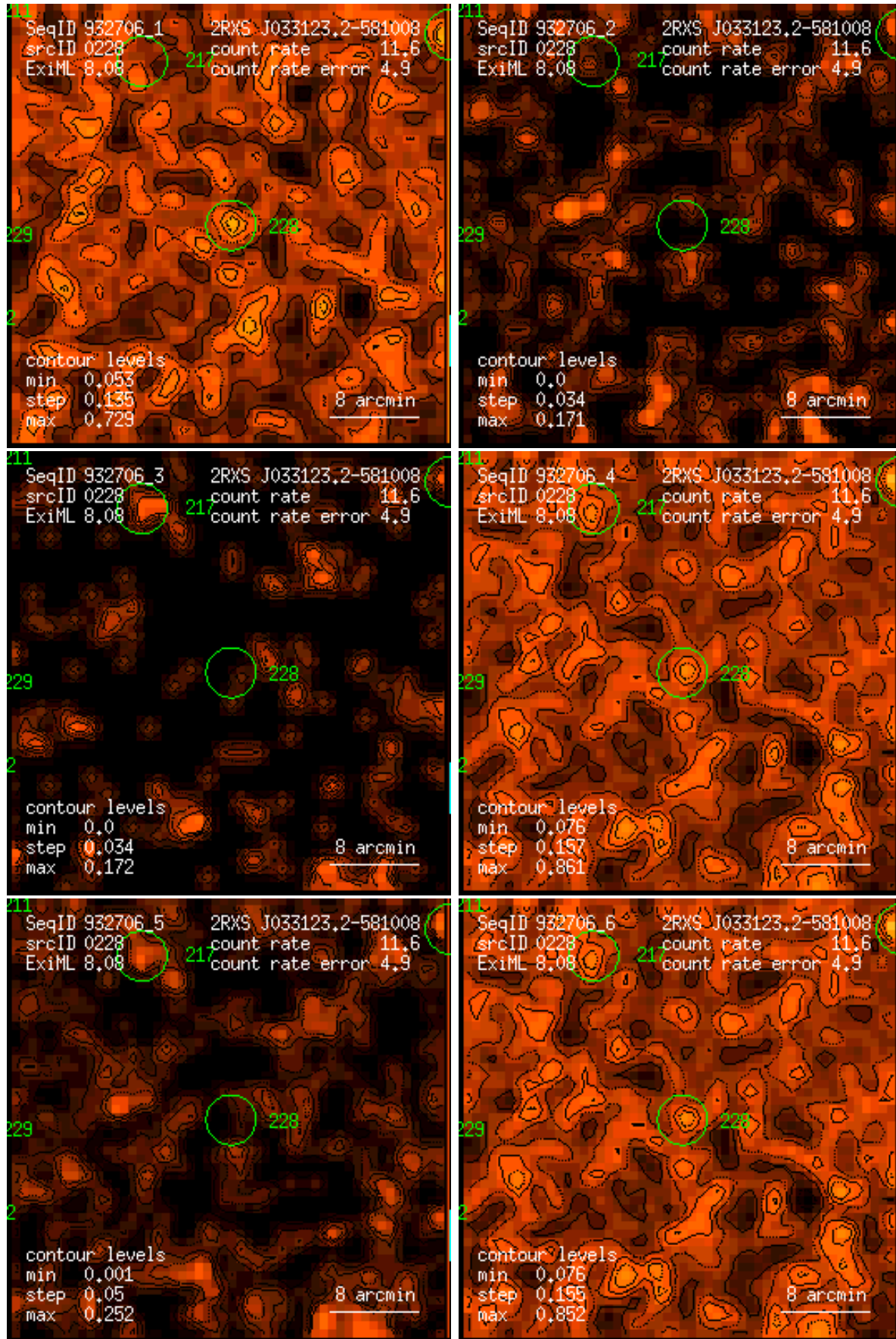
Figure 228: RASS 932706: detection 0228: band rate images, Gaussian filter: (1) PSPC channels 11 – 41, (2) 52 – 90, (3) 91 – 201, (4) 11 – 235, (5) 52 – 201, (6) 11 – 201. Broad band rates in counts/ks. Band rate contour levels in counts/ks/arcmin 2 .
