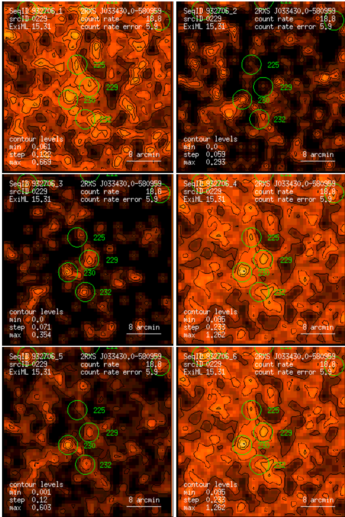
Figure 229: RASS 932706: detection 0229: band rate images, Gaussian filter: (1) PSPC channels 11 – 41, (2) 52 – 90, (3) 91 – 201, (4) 11 – 235, (5) 52 – 201, (6) 11 – 201. Broad band rates in counts/ks. Band rate contour levels in counts/ks/arcmin 2 .
