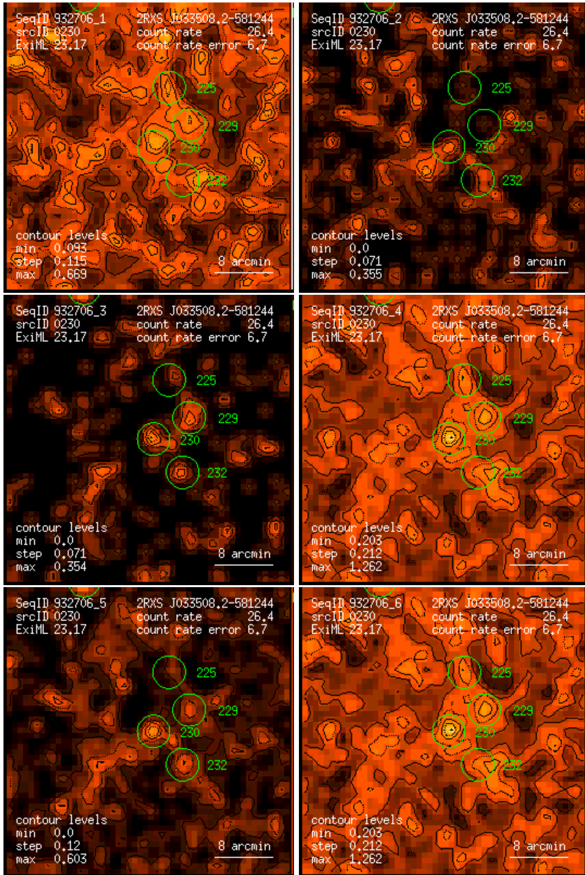
Figure 230: RASS 932706: detection 0230: band rate images, Gaussian filter: (1) PSPC channels 11 – 41, (2) 52 – 90, (3) 91 – 201, (4) 11 – 235, (5) 52 – 201, (6) 11 – 201. Broad band rates in counts/ks. Band rate contour levels in counts/ks/arcmin 2 .
