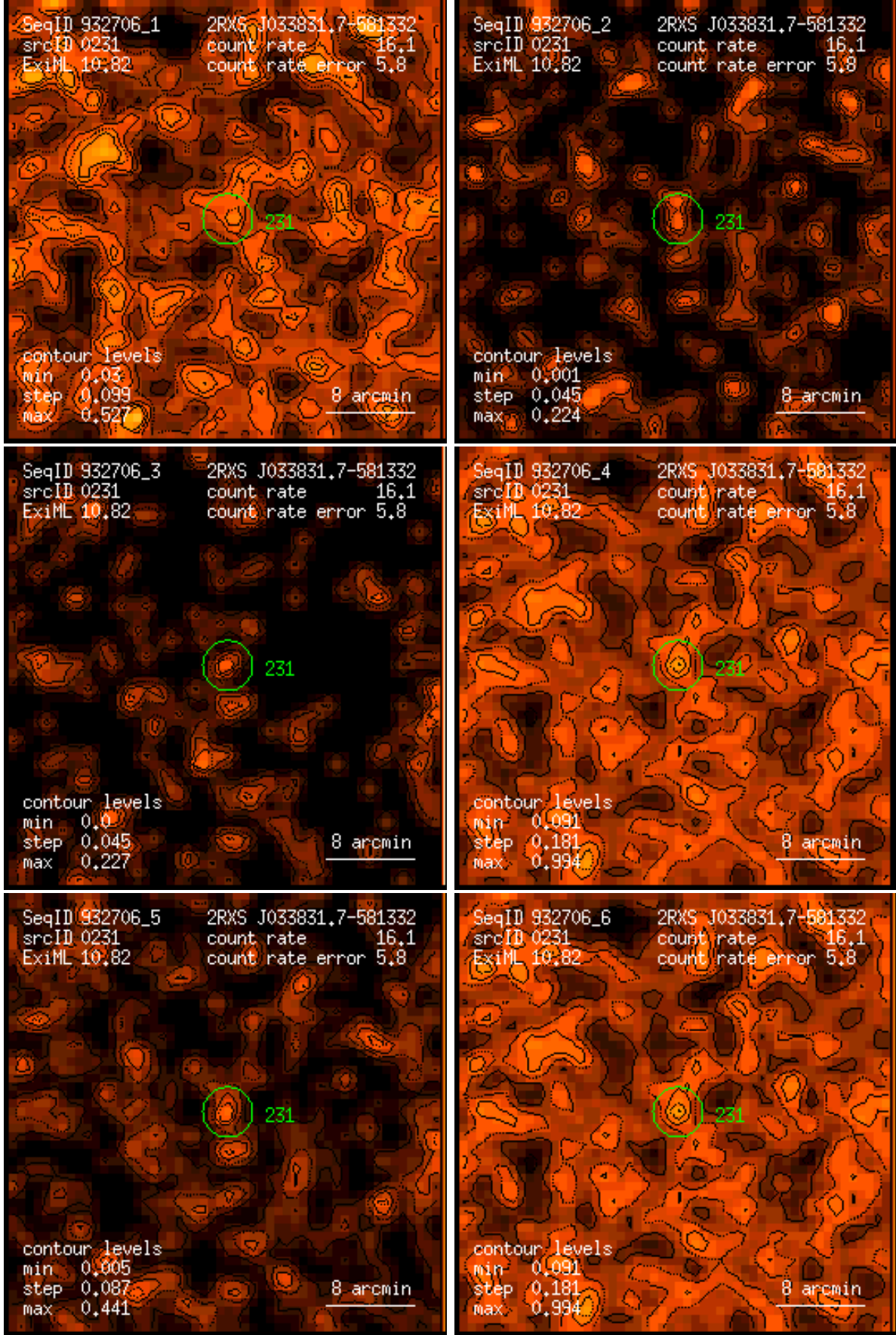
Figure 231: RASS 932706: detection 0231: band rate images, Gaussian filter: (1) PSPC channels 11 – 41, (2) 52 – 90, (3) 91 – 201, (4) 11 – 235, (5) 52 – 201, (6) 11 – 201. Broad band rates in counts/ks. Band rate contour levels in counts/ks/arcmin 2 .
