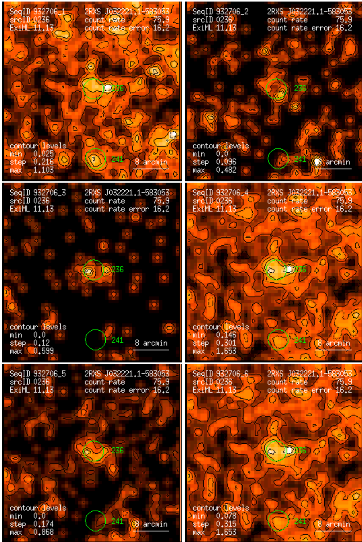
Figure 236: RASS 932706: detection 0236: band rate images, Gaussian filter: (1) PSPC channels 11 – 41, (2) 52 – 90, (3) 91 – 201, (4) 11 – 235, (5) 52 – 201, (6) 11 – 201. Broad band rates in counts/ks. Band rate contour levels in counts/ks/arcmin 2 .
