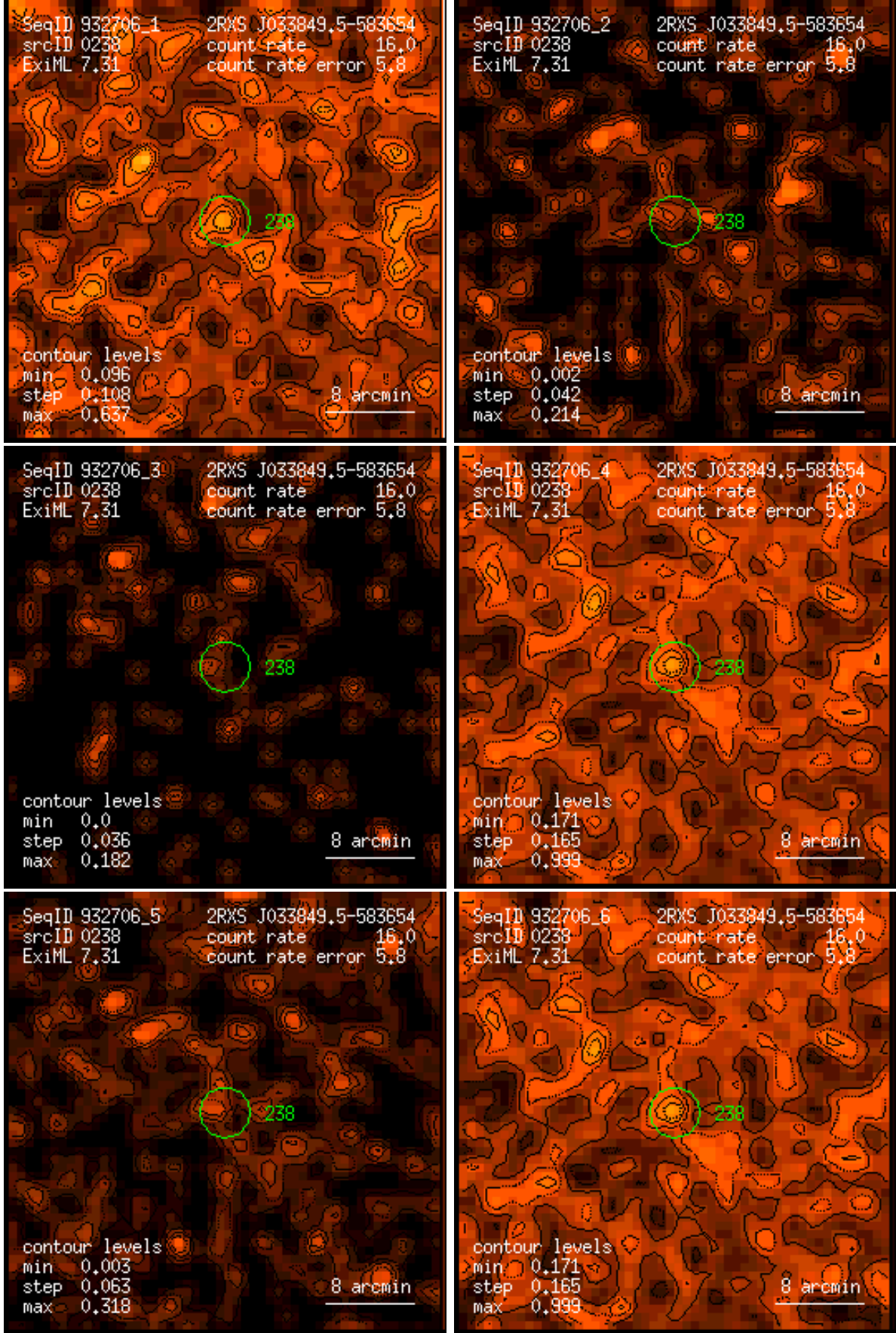
Figure 238: RASS 932706: detection 0238: band rate images, Gaussian filter: (1) PSPC channels 11 – 41, (2) 52 – 90, (3) 91 – 201, (4) 11 – 235, (5) 52 – 201, (6) 11 – 201. Broad band rates in counts/ks. Band rate contour levels in counts/ks/arcmin 2 .
