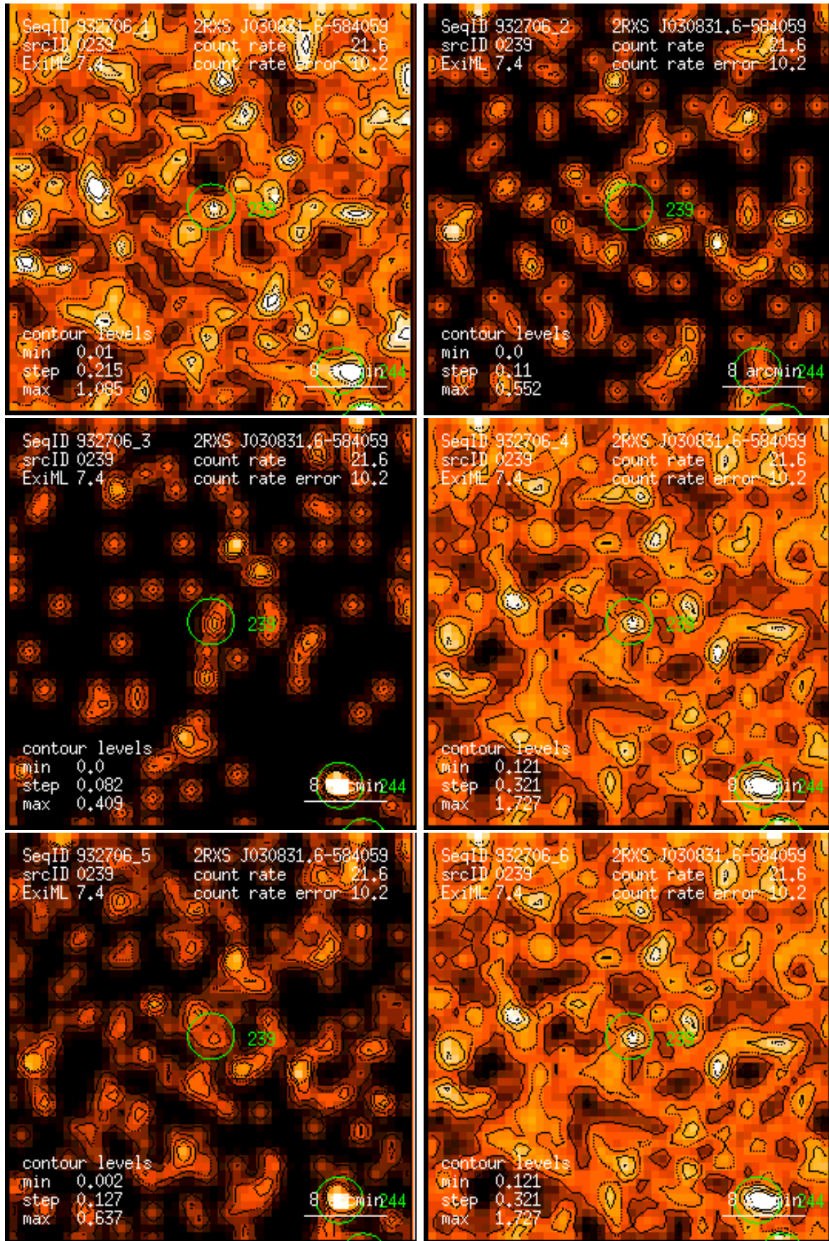
Figure 239: RASS 932706: detection 0239: band rate images, Gaussian filter: (1) PSPC channels 11 – 41, (2) 52 – 90, (3) 91 – 201, (4) 11 – 235, (5) 52 – 201, (6) 11 – 201. Broad band rates in counts/ks. Band rate contour levels in counts/ks/arcmin 2 .
