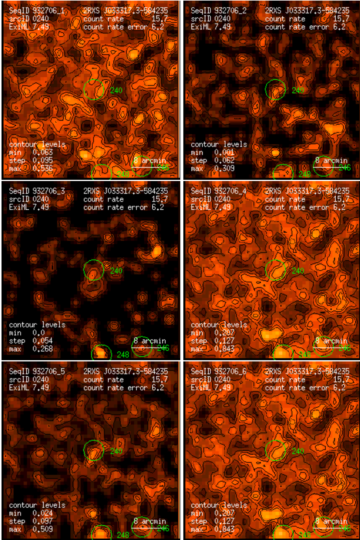
Figure 240: RASS 932706: detection 0240: band rate images, Gaussian filter: (1) PSPC channels 11 – 41, (2) 52 – 90, (3) 91 – 201, (4) 11 – 235, (5) 52 – 201, (6) 11 – 201. Broad band rates in counts/ks. Band rate contour levels in counts/ks/arcmin 2 .
