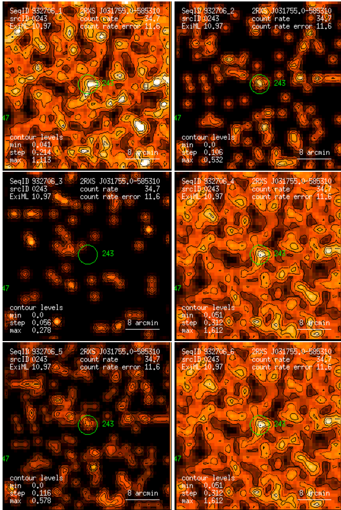
Figure 243: RASS 932706: detection 0243: band rate images, Gaussian filter: (1) PSPC channels 11 – 41, (2) 52 – 90, (3) 91 – 201, (4) 11 – 235, (5) 52 – 201, (6) 11 – 201. Broad band rates in counts/ks. Band rate contour levels in counts/ks/arcmin 2 .
