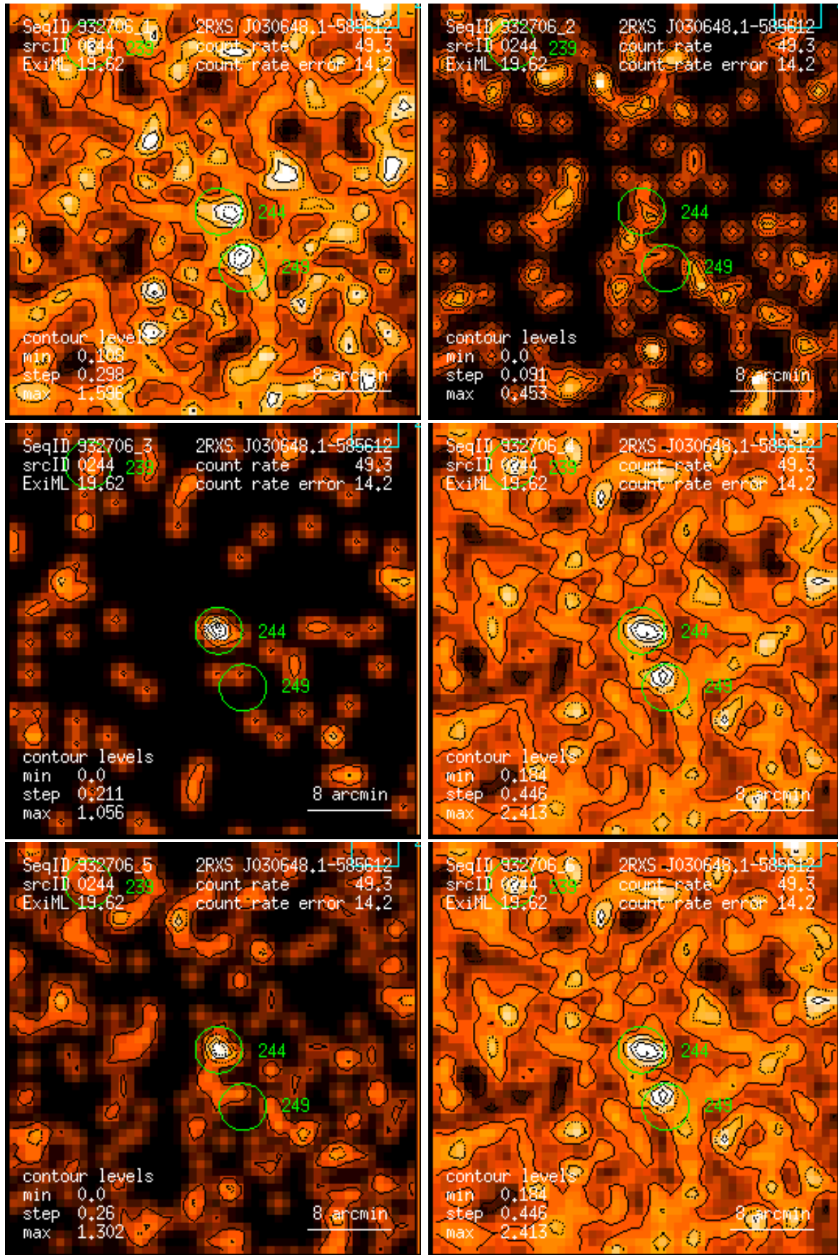
Figure 244: RASS 932706: detection 0244: band rate images, Gaussian filter: (1) PSPC channels 11 – 41, (2) 52 – 90, (3) 91 – 201, (4) 11 – 235, (5) 52 – 201, (6) 11 – 201. Broad band rates in counts/ks. Band rate contour levels in counts/ks/arcmin 2 .
