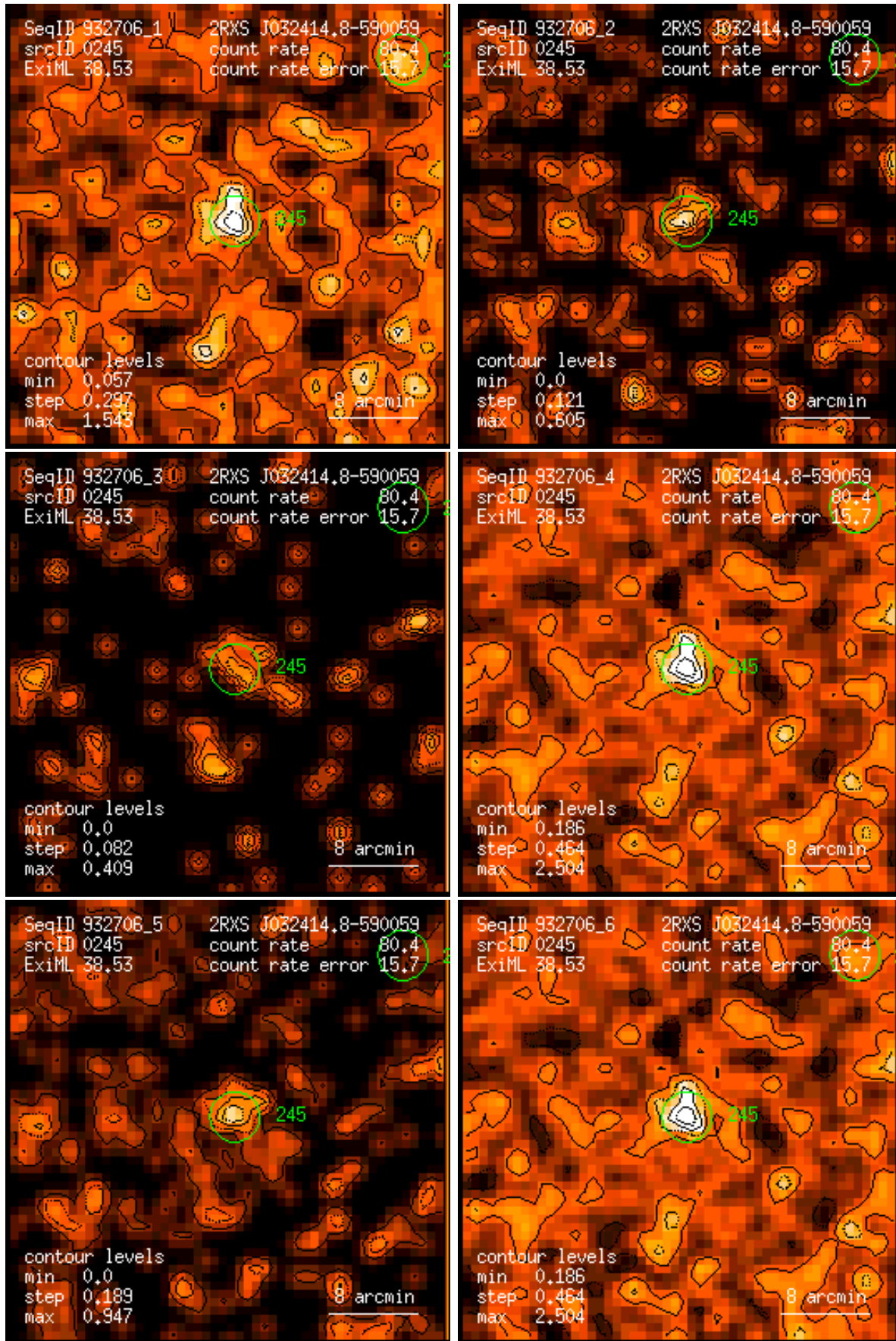
Figure 245: RASS 932706: detection 0245: band rate images, Gaussian filter: (1) PSPC channels 11 – 41, (2) 52 – 90, (3) 91 – 201, (4) 11 – 235, (5) 52 – 201, (6) 11 – 201. Broad band rates in counts/ks. Band rate contour levels in counts/ks/arcmin 2 .
