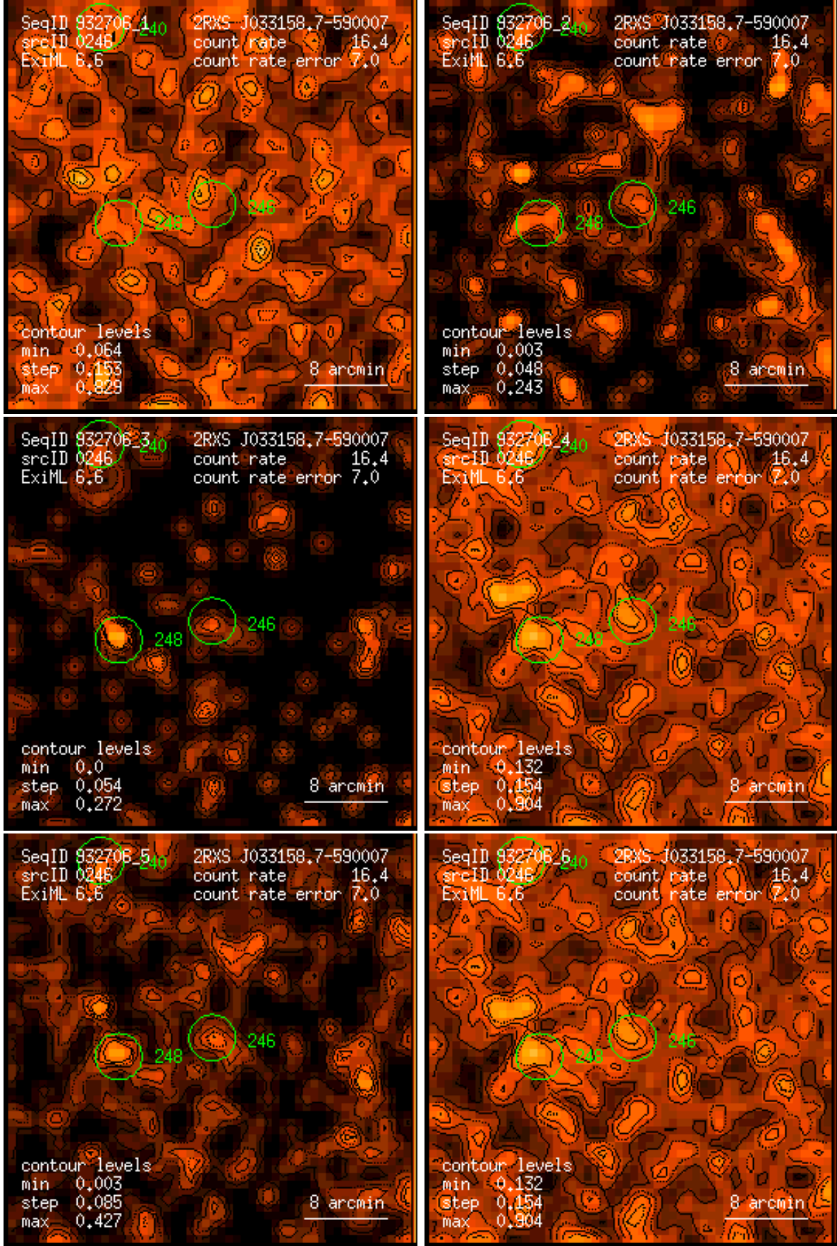
Figure 246: RASS 932706: detection 0246: band rate images, Gaussian filter: (1) PSPC channels 11 – 41, (2) 52 – 90, (3) 91 – 201, (4) 11 – 235, (5) 52 – 201, (6) 11 – 201. Broad band rates in counts/ks. Band rate contour levels in counts/ks/arcmin 2 .
