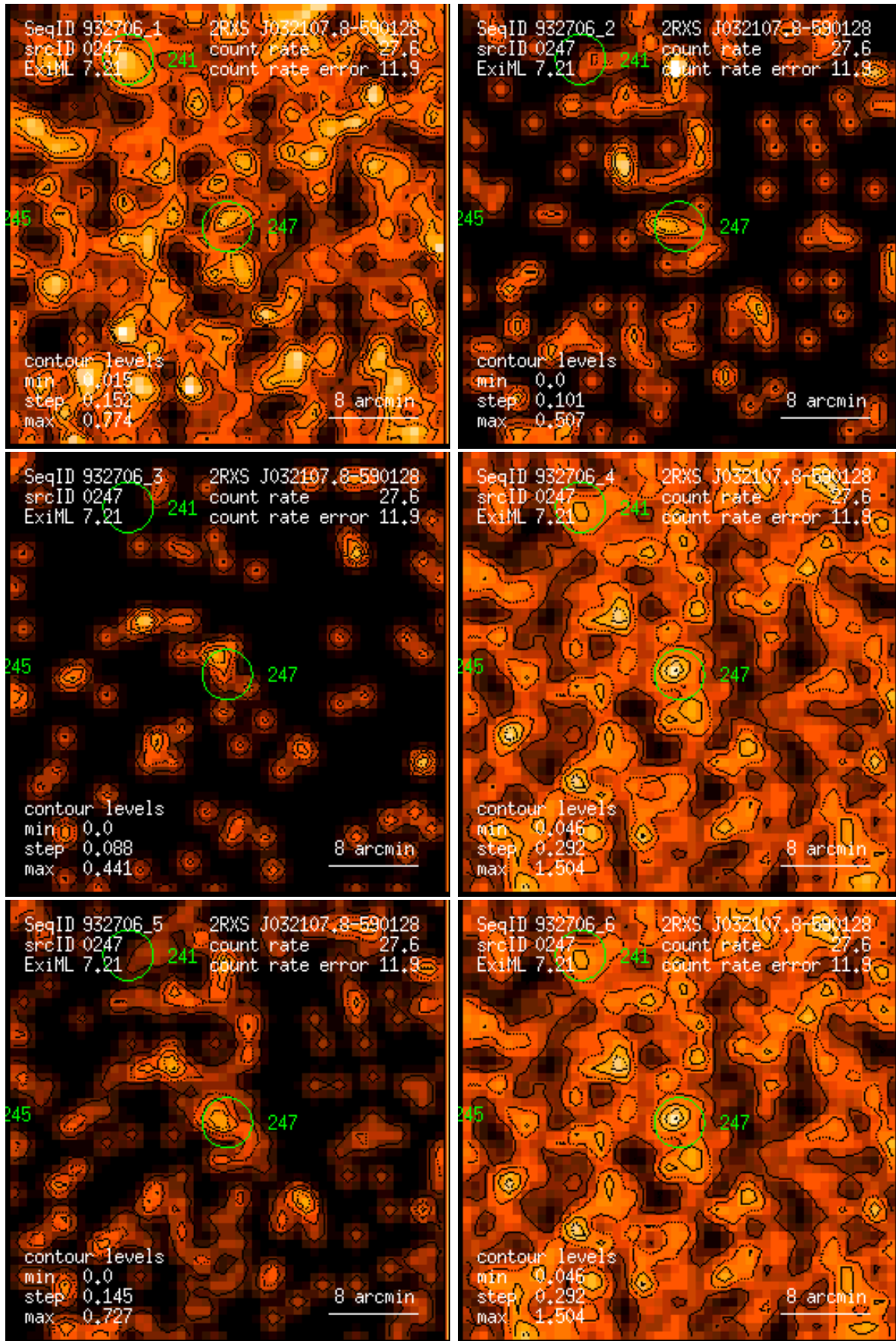
Figure 247: RASS 932706: detection 0247: band rate images, Gaussian filter: (1) PSPC channels 11 – 41, (2) 52 – 90, (3) 91 – 201, (4) 11 – 235, (5) 52 – 201, (6) 11 – 201. Broad band rates in counts/ks. Band rate contour levels in counts/ks/arcmin 2 .
