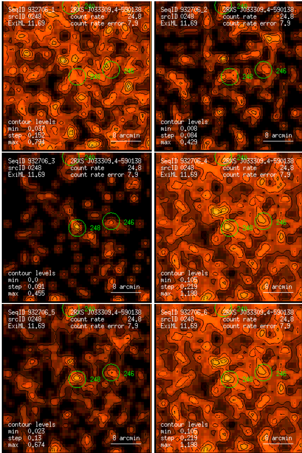
Figure 248: RASS 932706: detection 0248: band rate images, Gaussian filter: (1) PSPC channels 11 – 41, (2) 52 – 90, (3) 91 – 201, (4) 11 – 235, (5) 52 – 201, (6) 11 – 201. Broad band rates in counts/ks. Band rate contour levels in counts/ks/arcmin 2 .
