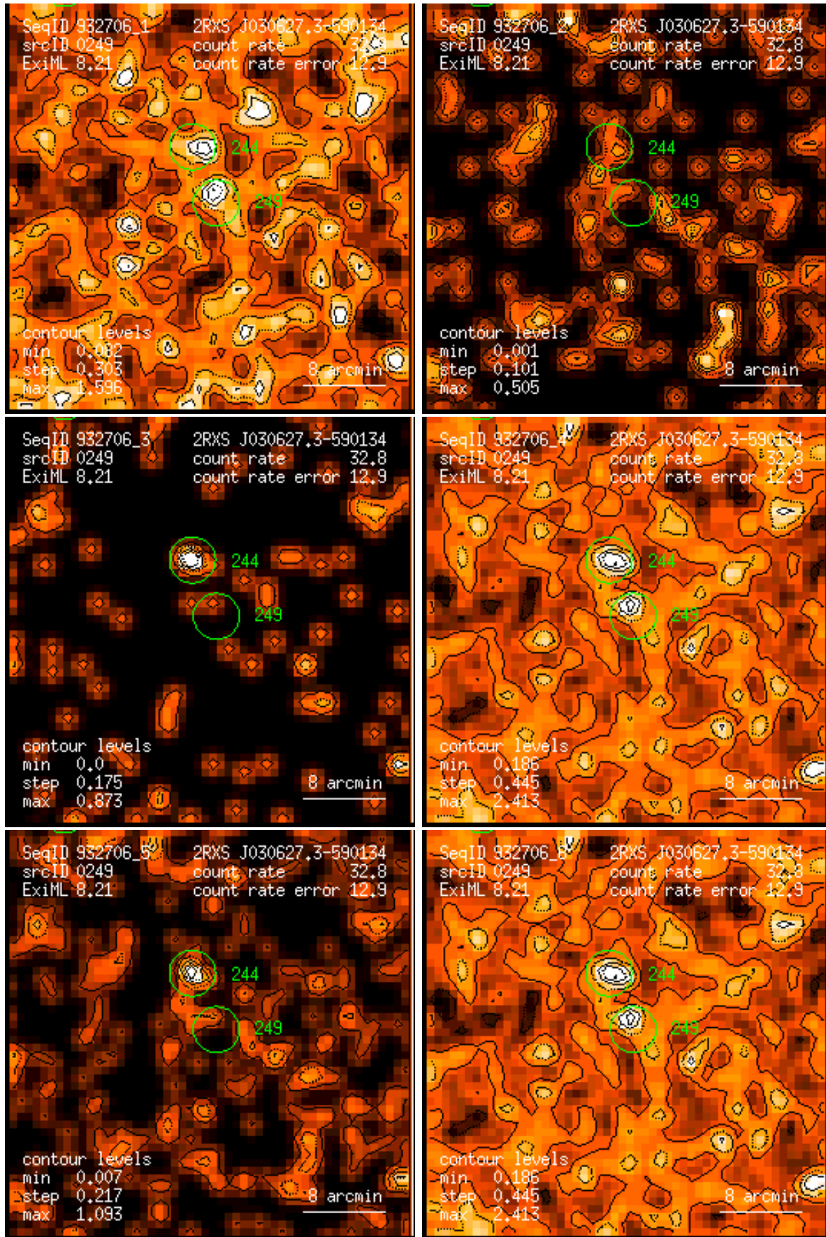
Figure 249: RASS 932706: detection 0249: band rate images, Gaussian filter: (1) PSPC channels 11 – 41, (2) 52 – 90, (3) 91 – 201, (4) 11 – 235, (5) 52 – 201, (6) 11 – 201. Broad band rates in counts/ks. Band rate contour levels in counts/ks/arcmin 2 .
