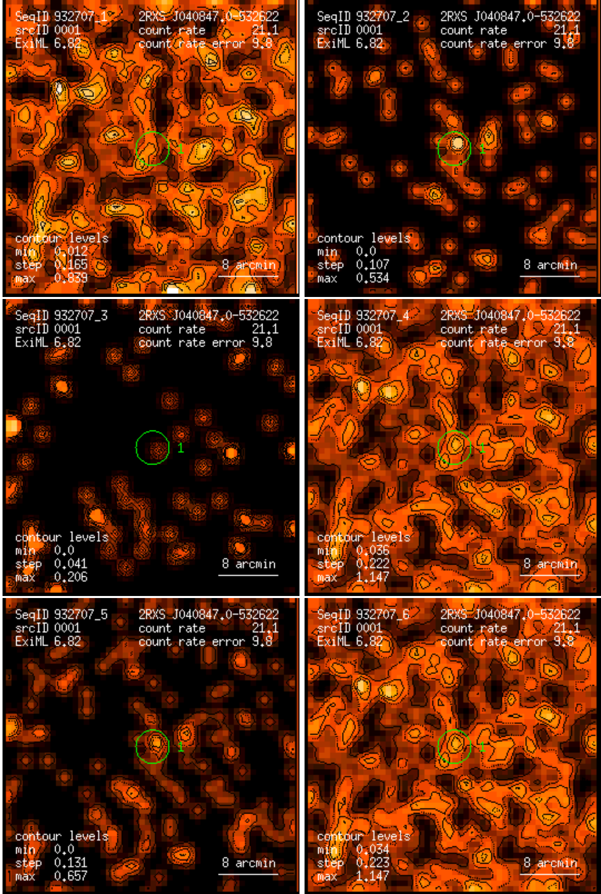
Figure 1: RASS 932707: detection 0001: band rate images, Gaussian filter: (1) PSPC channels 11 – 41, (2) 52 – 90, (3) 91 – 201, (4) 11 – 235, (5) 52 – 201, (6) 11 – 201. Broad band rates in counts/ks. Band rate contour levels in counts/ks/arcmin 2 .
