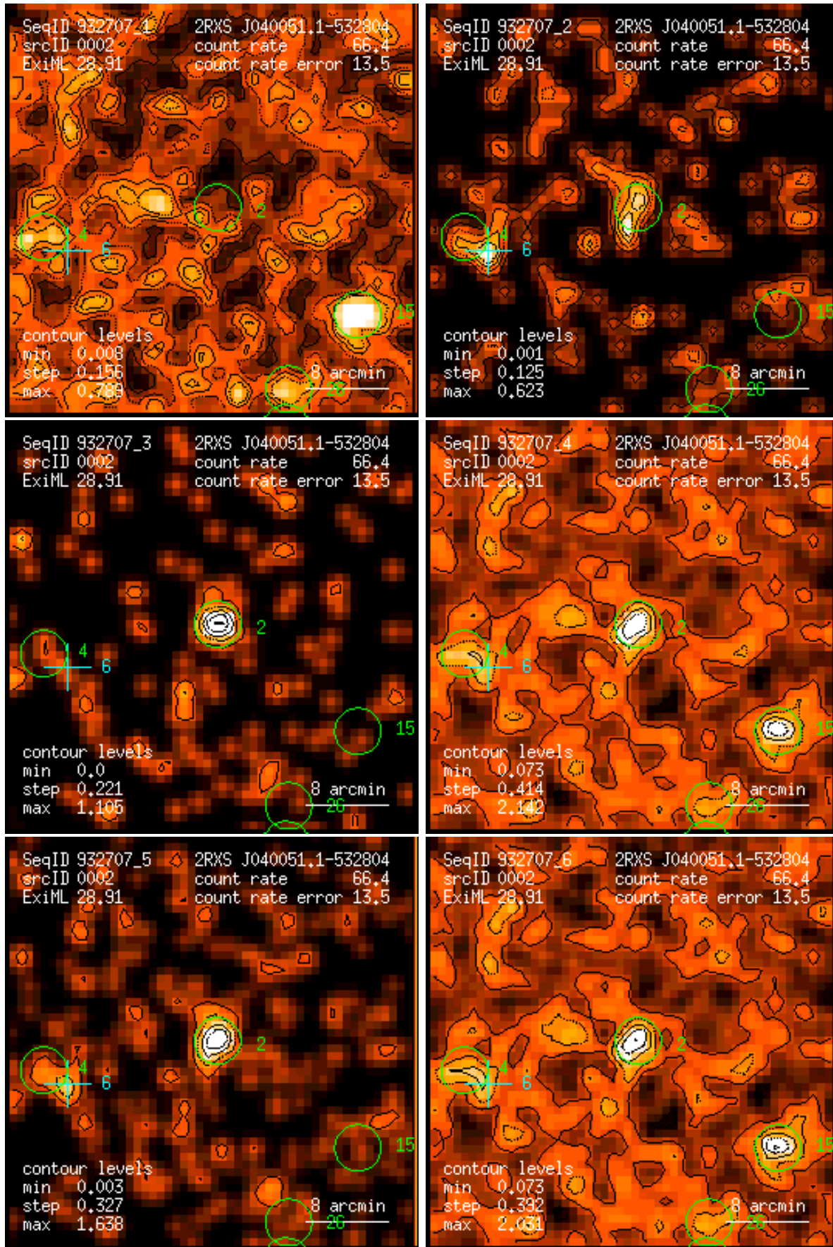
Figure 2: RASS 932707: detection 0002: band rate images, Gaussian filter: (1) PSPC channels 11 – 41, (2) 52 – 90, (3) 91 – 201, (4) 11 – 235, (5) 52 – 201, (6) 11 – 201. Broad band rates in counts/ks. Band rate contour levels in counts/ks/arcmin 2 .
