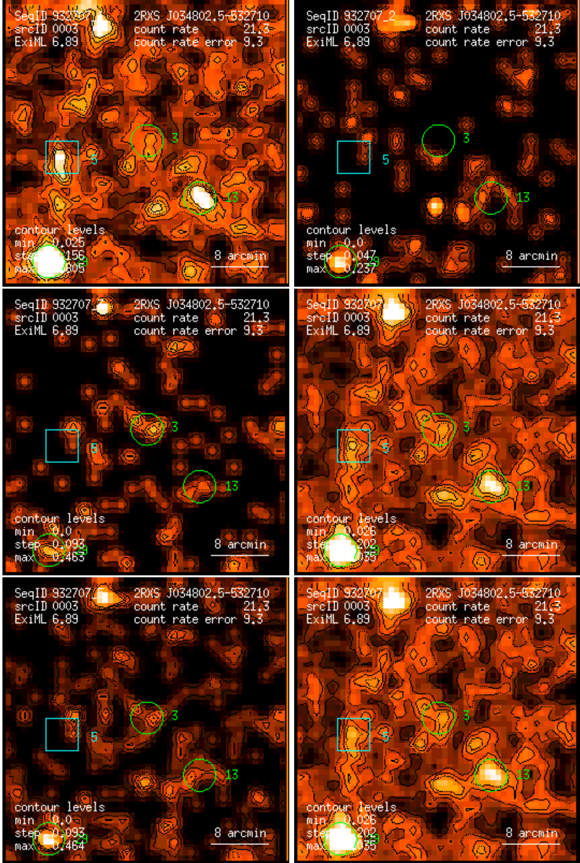
Figure 3: RASS 932707: detection 0003: band rate images, Gaussian filter: (1) PSPC channels 11 – 41, (2) 52 – 90, (3) 91 – 201, (4) 11 – 235, (5) 52 – 201, (6) 11 – 201. Broad band rates in counts/ks. Band rate contour levels in counts/ks/arcmin 2 .
