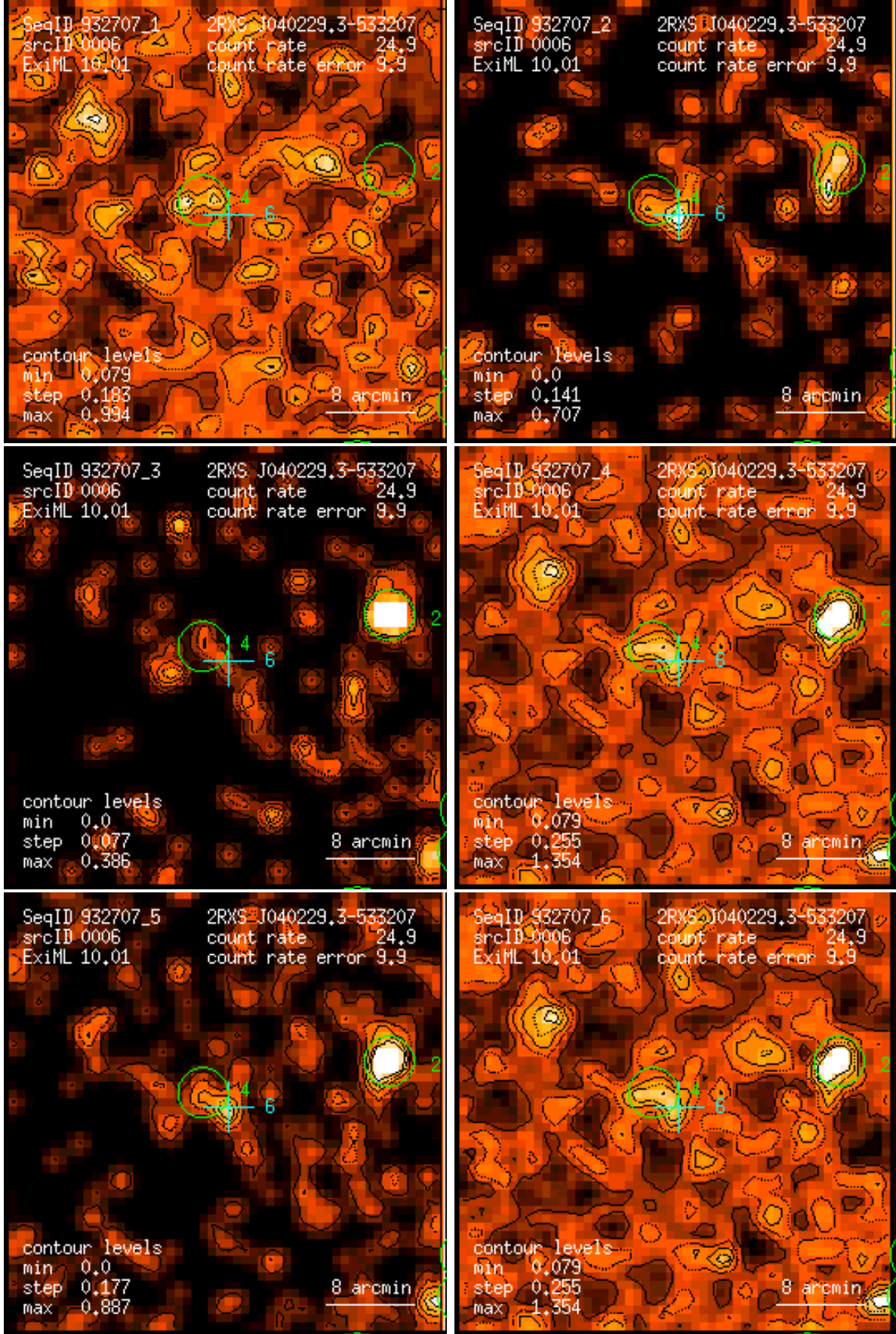
Figure 6: RASS 932707: detection 0006: band rate images, Gaussian filter: (1) PSPC channels 11 – 41, (2) 52 – 90, (3) 91 – 201, (4) 11 – 235, (5) 52 – 201, (6) 11 – 201. Broad band rates in counts/ks. Band rate contour levels in counts/ks/arcmin 2 .
