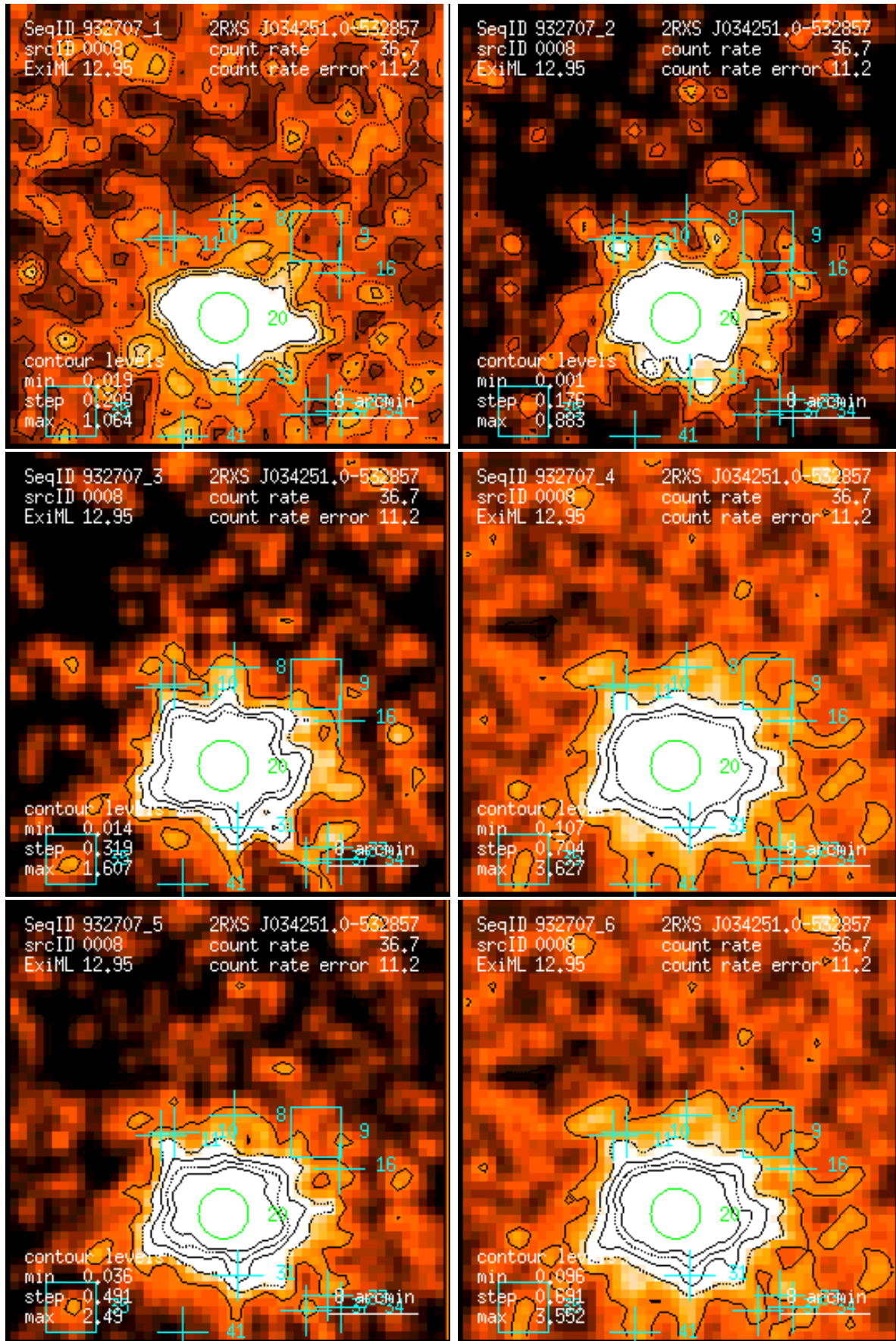
Figure 8: RASS 932707: detection 0008: band rate images, Gaussian filter: (1) PSPC channels 11 – 41, (2) 52 – 90, (3) 91 – 201, (4) 11 – 235, (5) 52 – 201, (6) 11 – 201. Broad band rates in counts/ks. Band rate contour levels in counts/ks/arcmin 2 .
