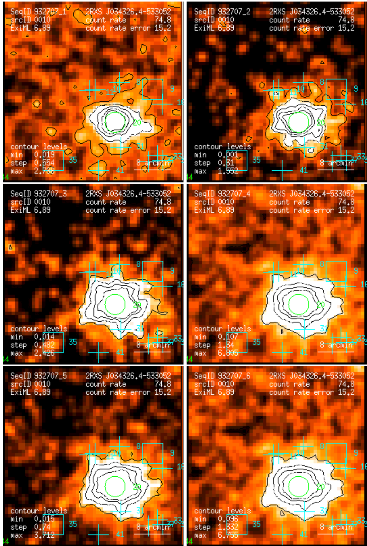
Figure 10: RASS 932707: detection 0010: band rate images, Gaussian filter: (1) PSPC channels 11 – 41, (2) 52 – 90, (3) 91 – 201, (4) 11 – 235, (5) 52 – 201, (6) 11 – 201. Broad band rates in counts/ks. Band rate contour levels in counts/ks/arcmin 2 .
