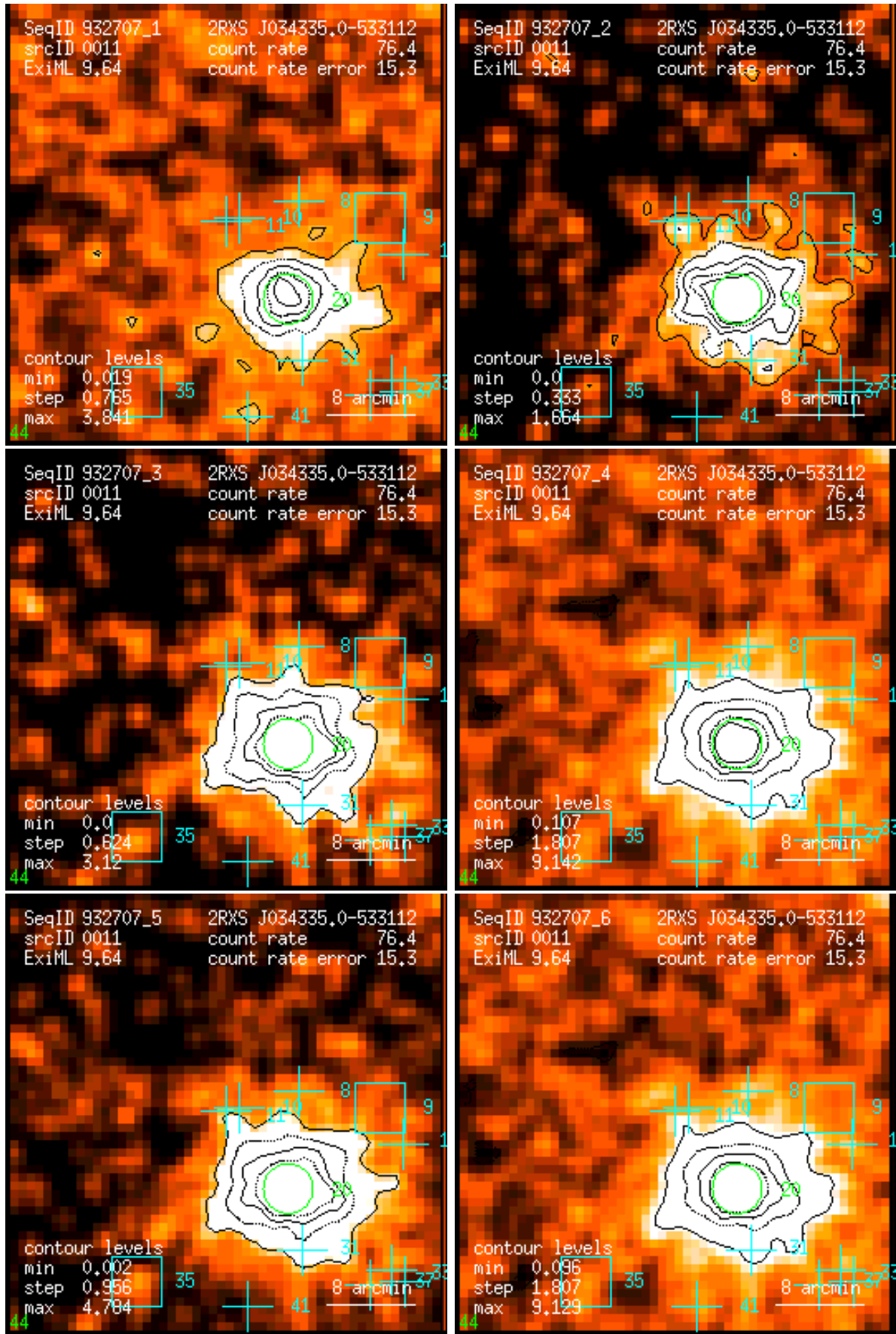
Figure 11: RASS 932707: detection 0011: band rate images, Gaussian filter: (1) PSPC channels 11 – 41, (2) 52 – 90, (3) 91 – 201, (4) 11 – 235, (5) 52 – 201, (6) 11 – 201. Broad band rates in counts/ks. Band rate contour levels in counts/ks/arcmin 2 .
