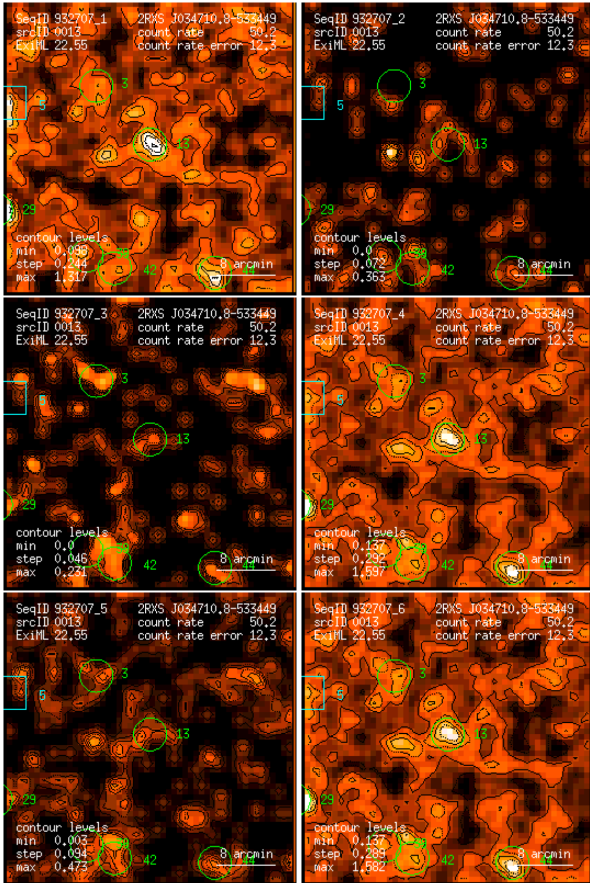
Figure 13: RASS 932707: detection 0013: band rate images, Gaussian filter: (1) PSPC channels 11 – 41, (2) 52 – 90, (3) 91 – 201, (4) 11 – 235, (5) 52 – 201, (6) 11 – 201. Broad band rates in counts/ks. Band rate contour levels in counts/ks/arcmin 2 .
