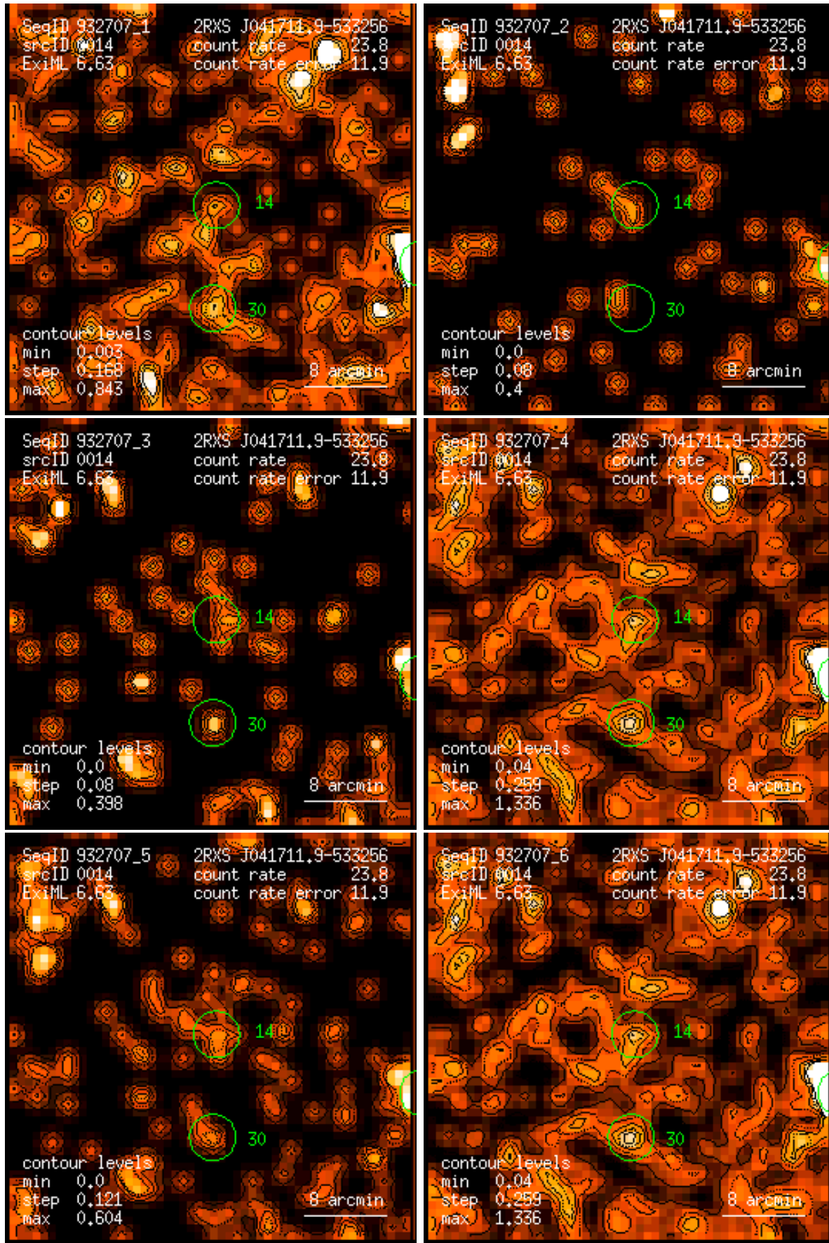
Figure 14: RASS 932707: detection 0014: band rate images, Gaussian filter: (1) PSPC channels 11 – 41, (2) 52 – 90, (3) 91 – 201, (4) 11 – 235, (5) 52 – 201, (6) 11 – 201. Broad band rates in counts/ks. Band rate contour levels in counts/ks/arcmin 2 .
