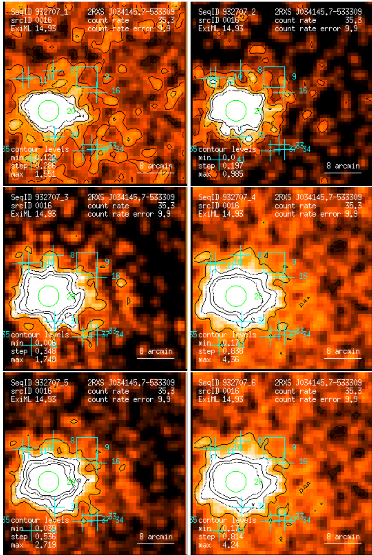
Figure 16: RASS 932707: detection 0016: band rate images, Gaussian filter: (1) PSPC channels 11 – 41, (2) 52 – 90, (3) 91 – 201, (4) 11 – 235, (5) 52 – 201, (6) 11 – 201. Broad band rates in counts/ks. Band rate contour levels in counts/ks/arcmin 2 .
