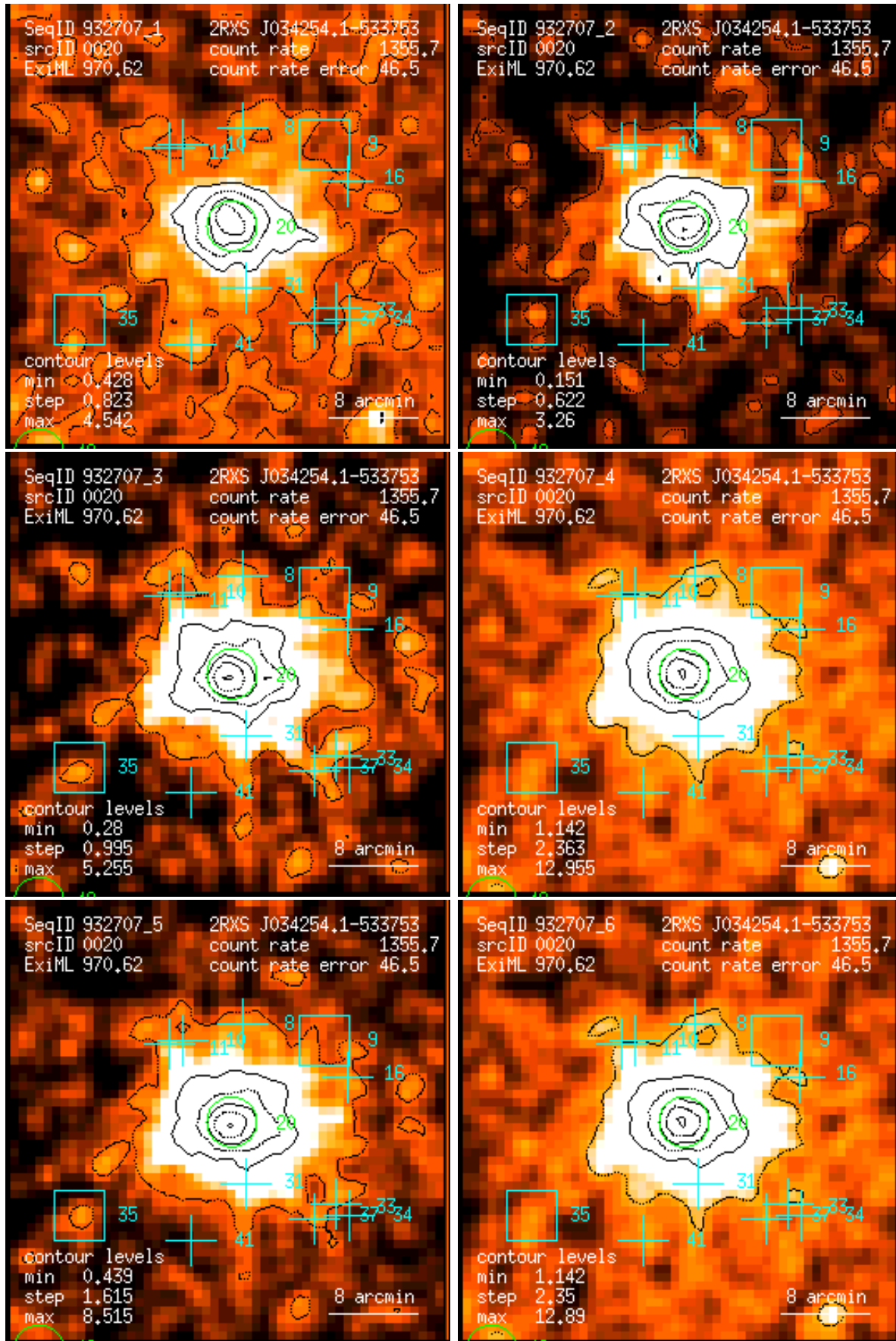
Figure 20: RASS 932707: detection 0020: band rate images, Gaussian filter: (1) PSPC channels 11 – 41, (2) 52 – 90, (3) 91 – 201, (4) 11 – 235, (5) 52 – 201, (6) 11 – 201. Broad band rates in counts/ks. Band rate contour levels in counts/ks/arcmin 2 .
