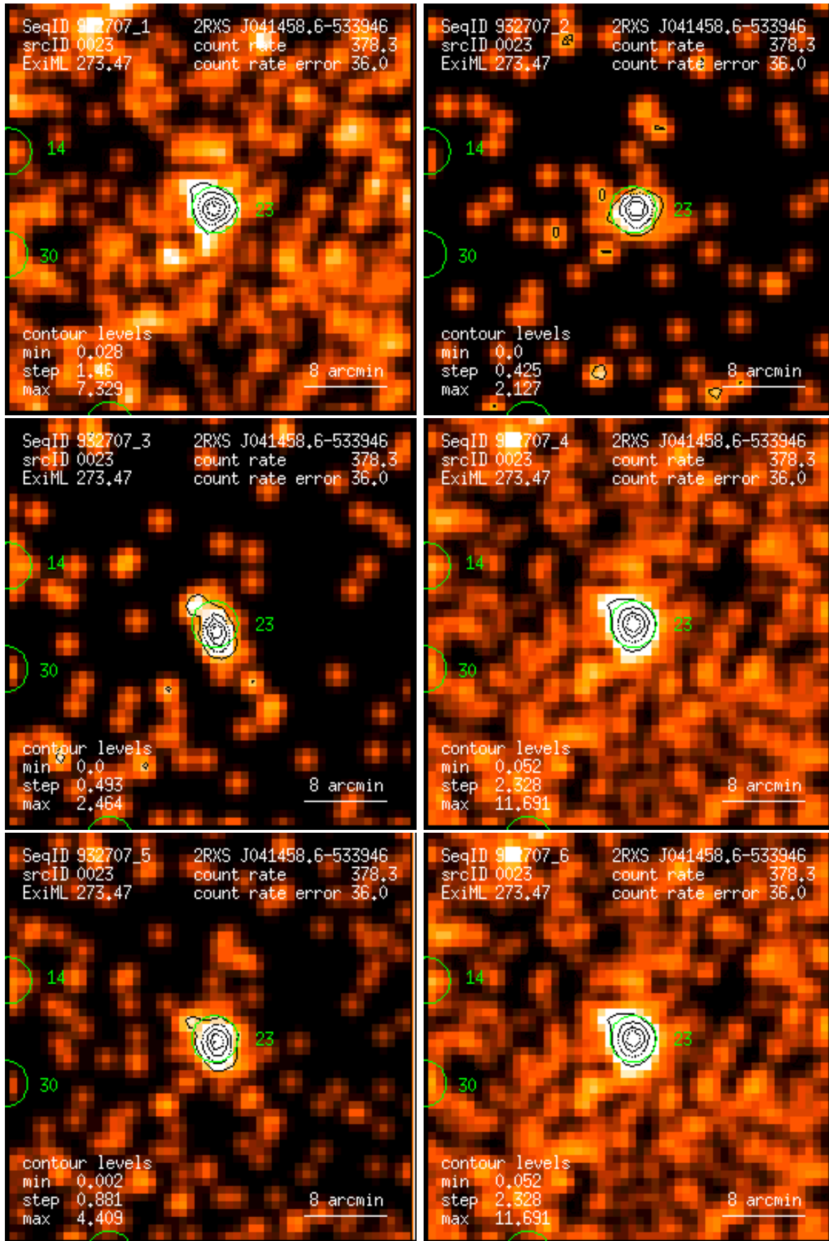
Figure 23: RASS 932707: detection 0023: band rate images, Gaussian filter: (1) PSPC channels 11 – 41, (2) 52 – 90, (3) 91 – 201, (4) 11 – 235, (5) 52 – 201, (6) 11 – 201. Broad band rates in counts/ks. Band rate contour levels in counts/ks/arcmin 2 .
