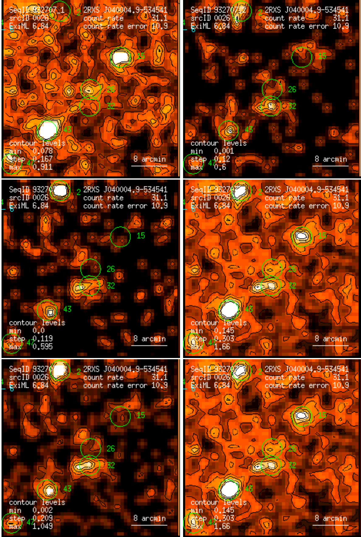
Figure 26: RASS 932707: detection 0026: band rate images, Gaussian filter: (1) PSPC channels 11 – 41, (2) 52 – 90, (3) 91 – 201, (4) 11 – 235, (5) 52 – 201, (6) 11 – 201. Broad band rates in counts/ks. Band rate contour levels in counts/ks/arcmin 2 .
