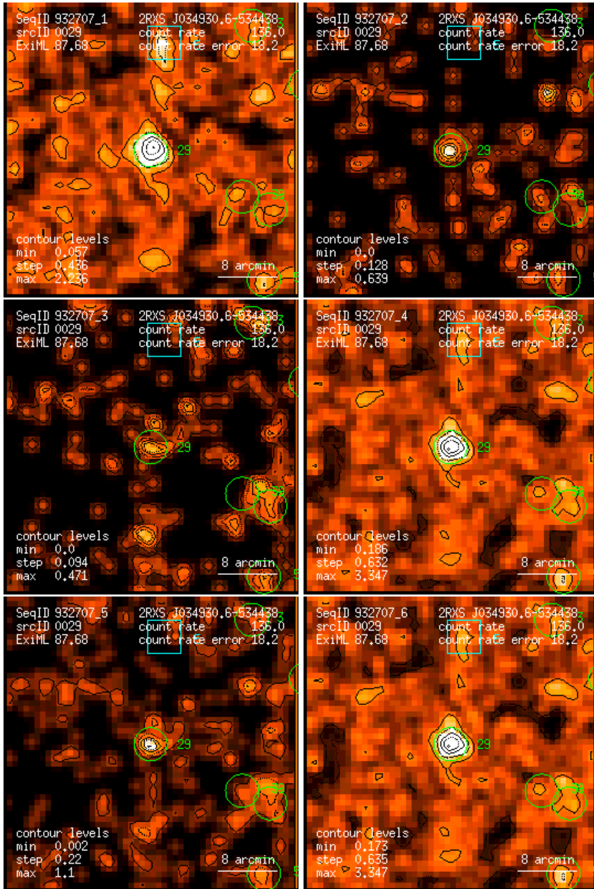
Figure 29: RASS 932707: detection 0029: band rate images, Gaussian filter: (1) PSPC channels 11 – 41, (2) 52 – 90, (3) 91 – 201, (4) 11 – 235, (5) 52 – 201, (6) 11 – 201. Broad band rates in counts/ks. Band rate contour levels in counts/ks/arcmin 2 .
