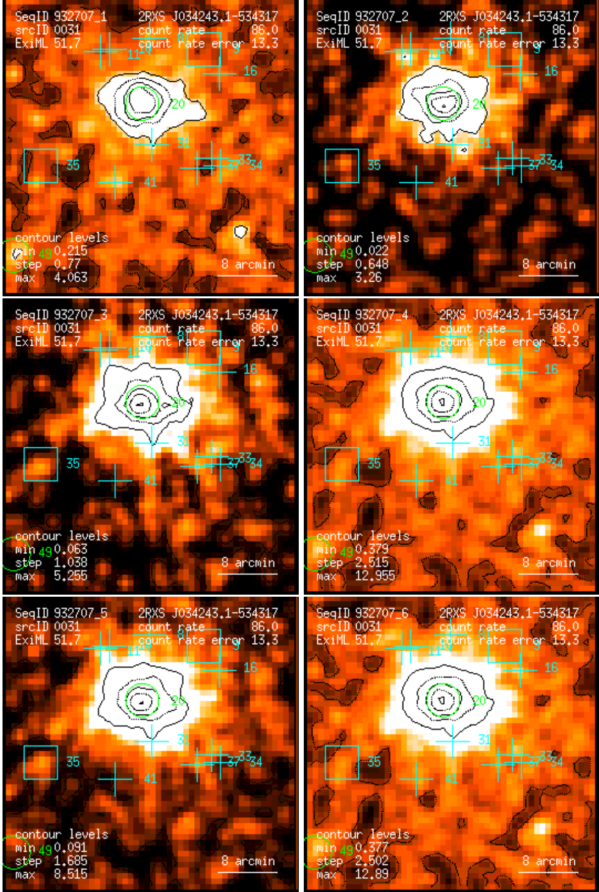
Figure 31: RASS 932707: detection 0031: band rate images, Gaussian filter: (1) PSPC channels 11 – 41, (2) 52 – 90, (3) 91 – 201, (4) 11 – 235, (5) 52 – 201, (6) 11 – 201. Broad band rates in counts/ks. Band rate contour levels in counts/ks/arcmin 2 .
