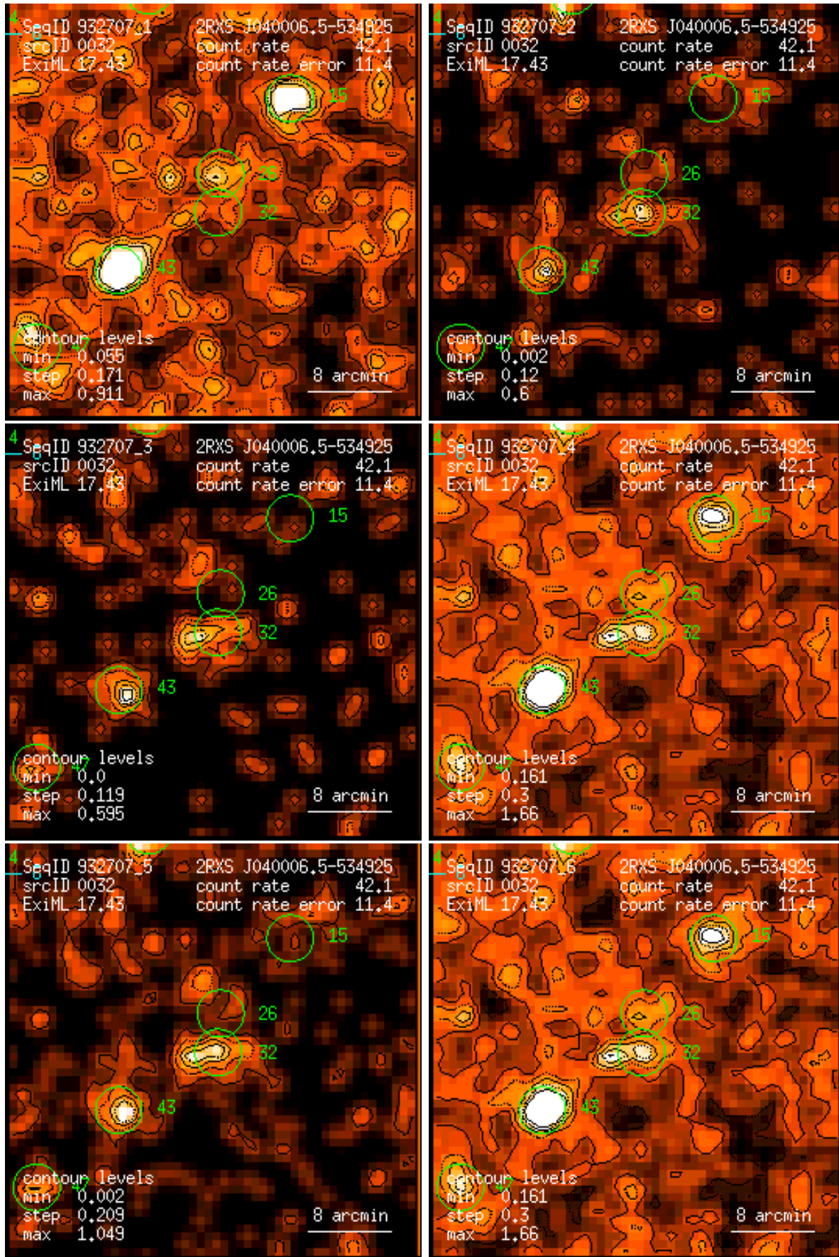
Figure 32: RASS 932707: detection 0032: band rate images, Gaussian filter: (1) PSPC channels 11 – 41, (2) 52 – 90, (3) 91 – 201, (4) 11 – 235, (5) 52 – 201, (6) 11 – 201. Broad band rates in counts/ks. Band rate contour levels in counts/ks/arcmin 2 .
