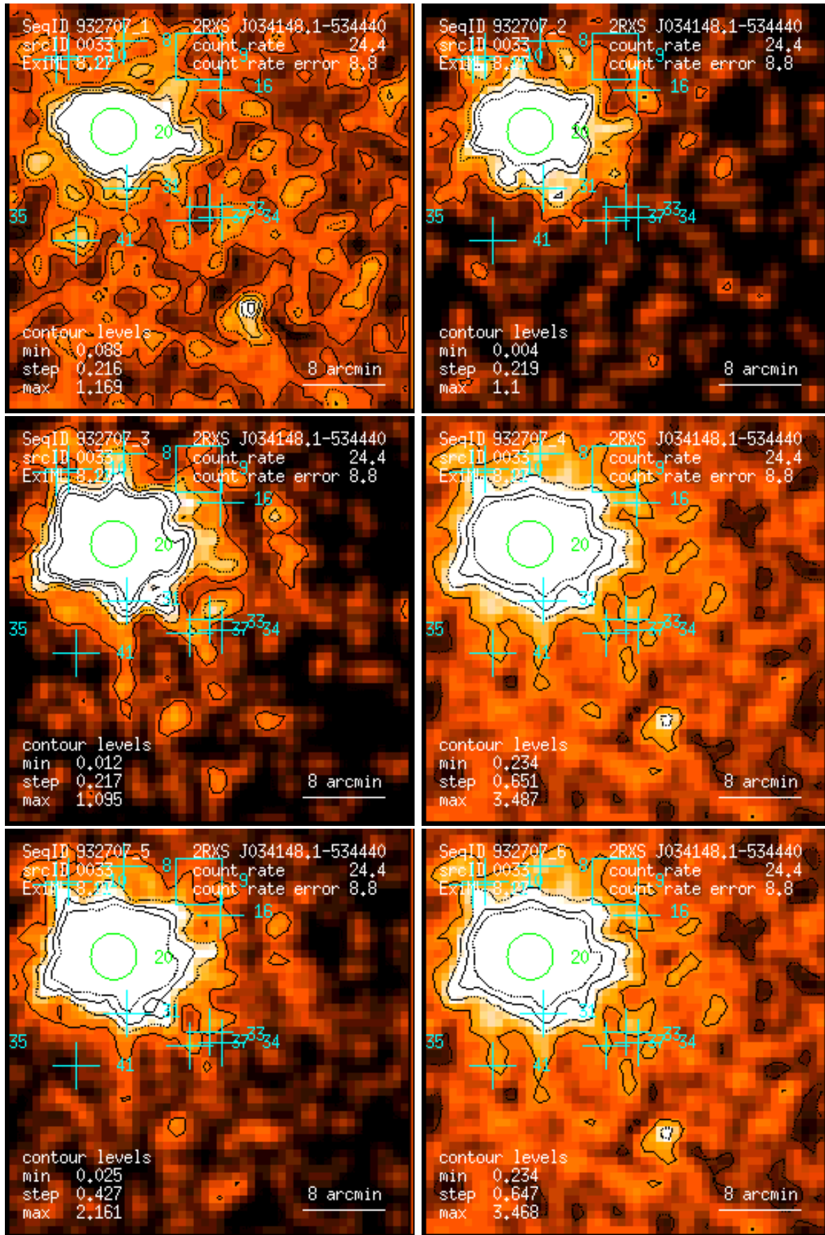
Figure 33: RASS 932707: detection 0033: band rate images, Gaussian filter: (1) PSPC channels 11 – 41, (2) 52 – 90, (3) 91 – 201, (4) 11 – 235, (5) 52 – 201, (6) 11 – 201. Broad band rates in counts/ks. Band rate contour levels in counts/ks/arcmin 2 .
