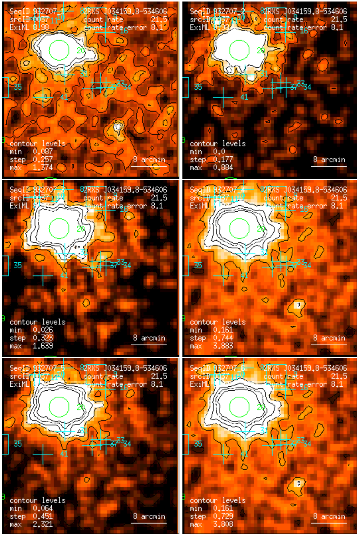
Figure 37: RASS 932707: detection 0037: band rate images, Gaussian filter: (1) PSPC channels 11 – 41, (2) 52 – 90, (3) 91 – 201, (4) 11 – 235, (5) 52 – 201, (6) 11 – 201. Broad band rates in counts/ks. Band rate contour levels in counts/ks/arcmin 2 .
