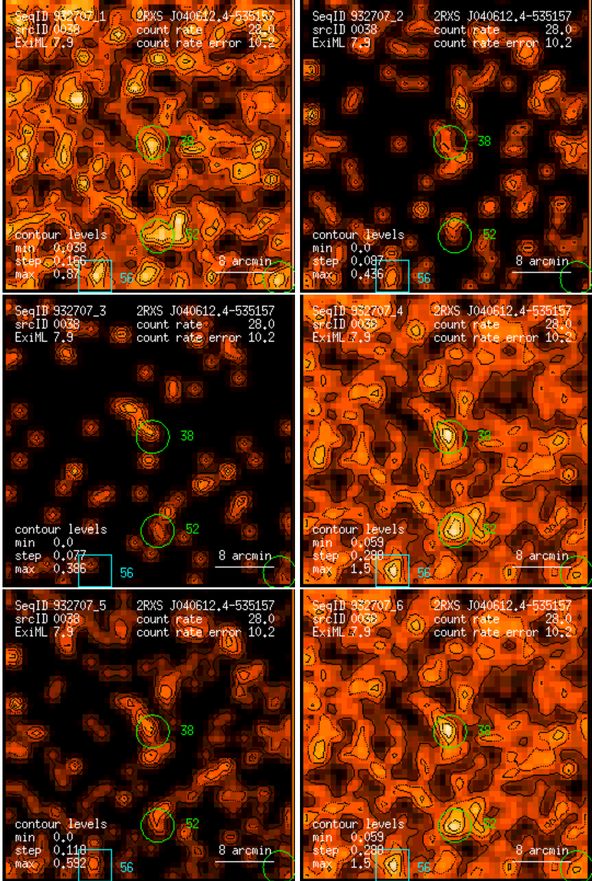
Figure 38: RASS 932707: detection 0038: band rate images, Gaussian filter: (1) PSPC channels 11 – 41, (2) 52 – 90, (3) 91 – 201, (4) 11 – 235, (5) 52 – 201, (6) 11 – 201. Broad band rates in counts/ks. Band rate contour levels in counts/ks/arcmin 2 .
