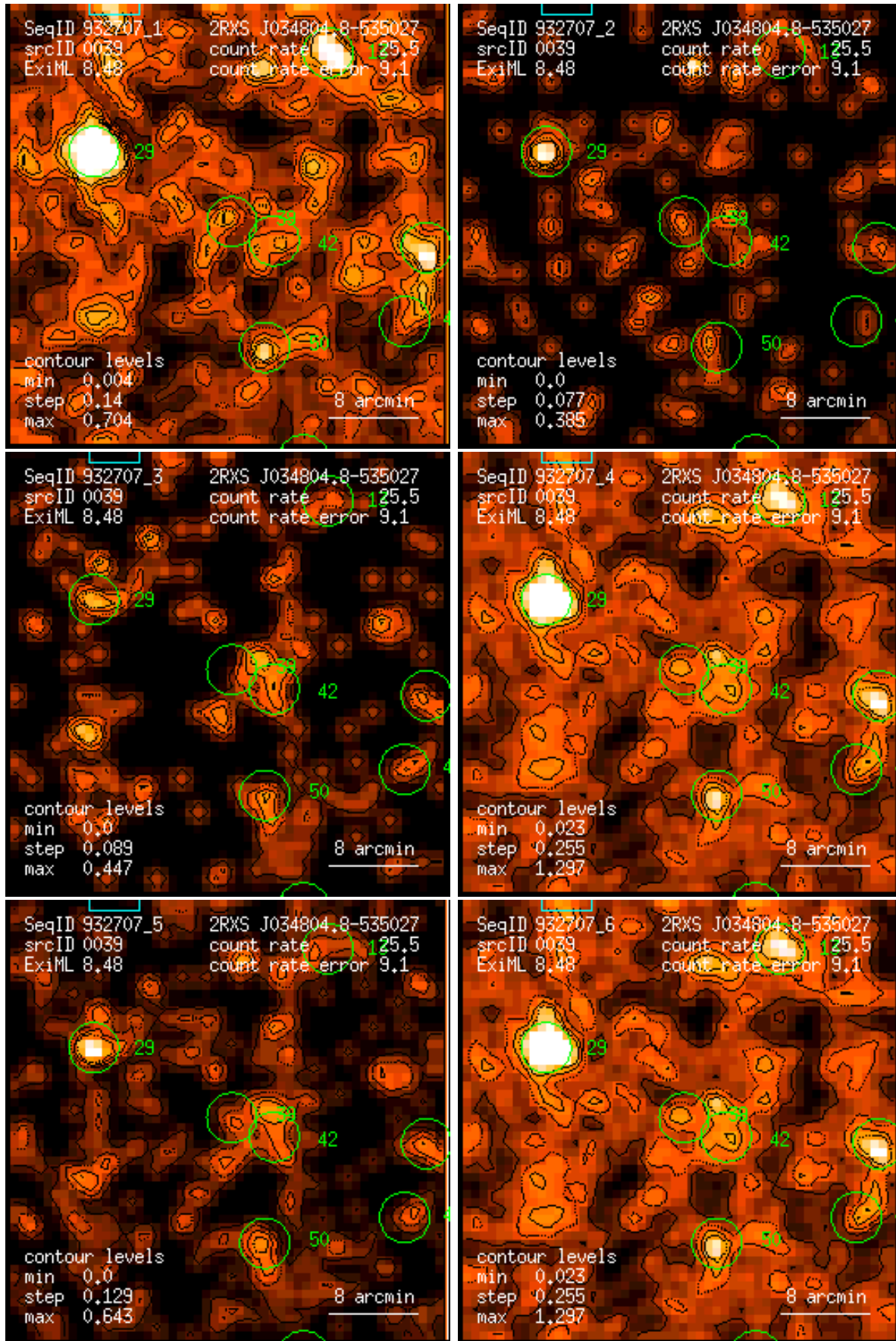
Figure 39: RASS 932707: detection 0039: band rate images, Gaussian filter: (1) PSPC channels 11 – 41, (2) 52 – 90, (3) 91 – 201, (4) 11 – 235, (5) 52 – 201, (6) 11 – 201. Broad band rates in counts/ks. Band rate contour levels in counts/ks/arcmin 2 .
