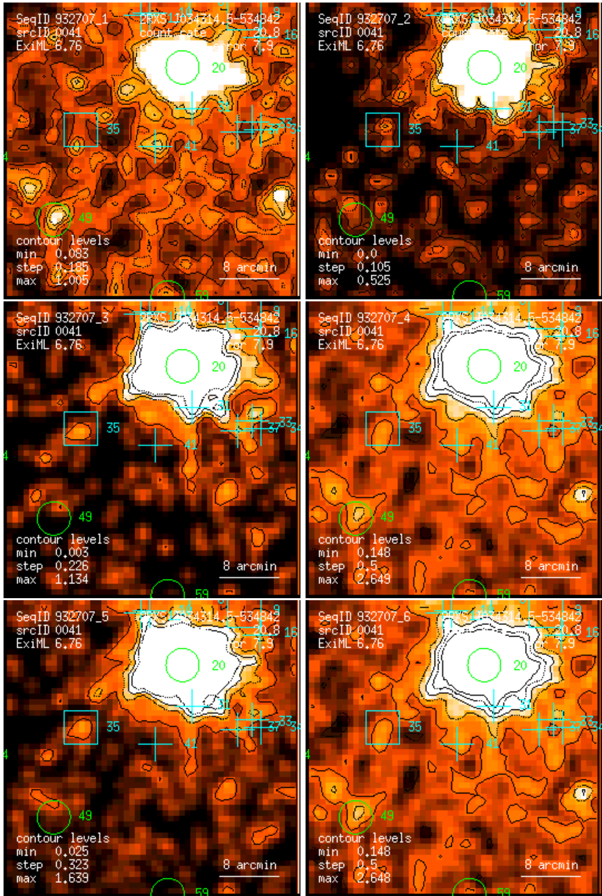
Figure 41: RASS 932707: detection 0041: band rate images, Gaussian filter: (1) PSPC channels 11 – 41, (2) 52 – 90, (3) 91 – 201, (4) 11 – 235, (5) 52 – 201, (6) 11 – 201. Broad band rates in counts/ks. Band rate contour levels in counts/ks/arcmin 2 .
