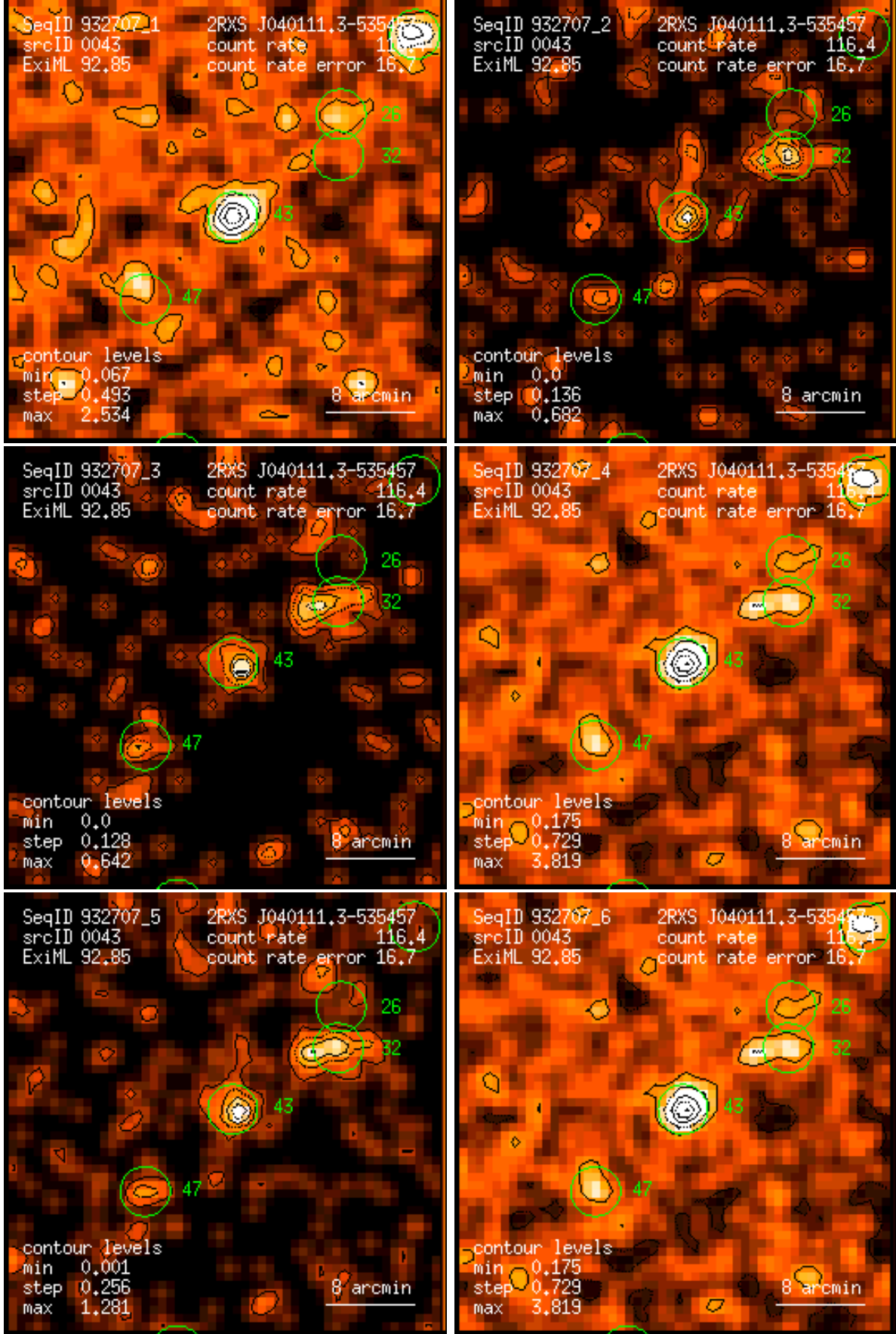
Figure 43: RASS 932707: detection 0043: band rate images, Gaussian filter: (1) PSPC channels 11 – 41, (2) 52 – 90, (3) 91 – 201, (4) 11 – 235, (5) 52 – 201, (6) 11 – 201. Broad band rates in counts/ks. Band rate contour levels in counts/ks/arcmin 2 .
