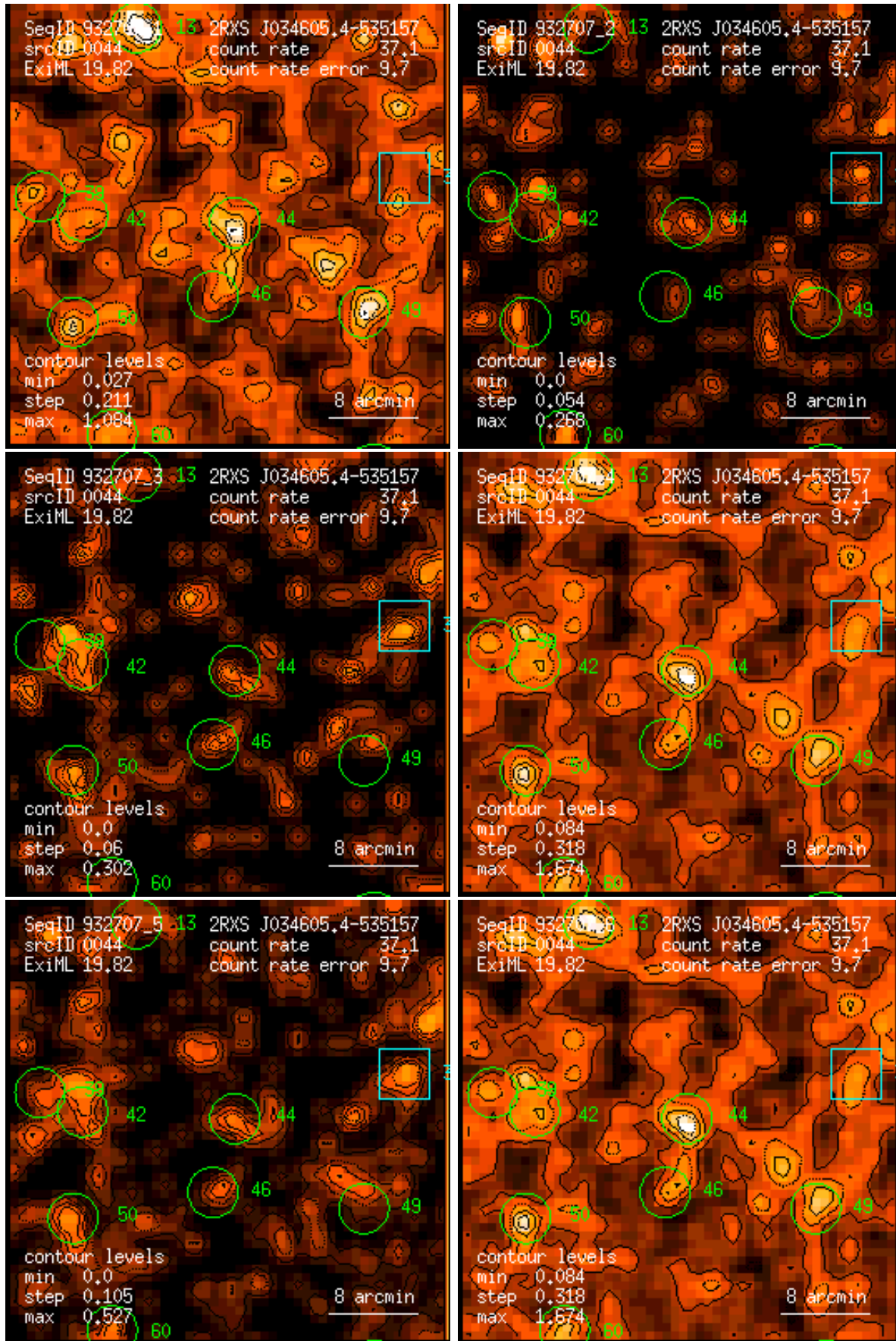
Figure 44: RASS 932707: detection 0044: band rate images, Gaussian filter: (1) PSPC channels 11 – 41, (2) 52 – 90, (3) 91 – 201, (4) 11 – 235, (5) 52 – 201, (6) 11 – 201. Broad band rates in counts/ks. Band rate contour levels in counts/ks/arcmin 2 .
