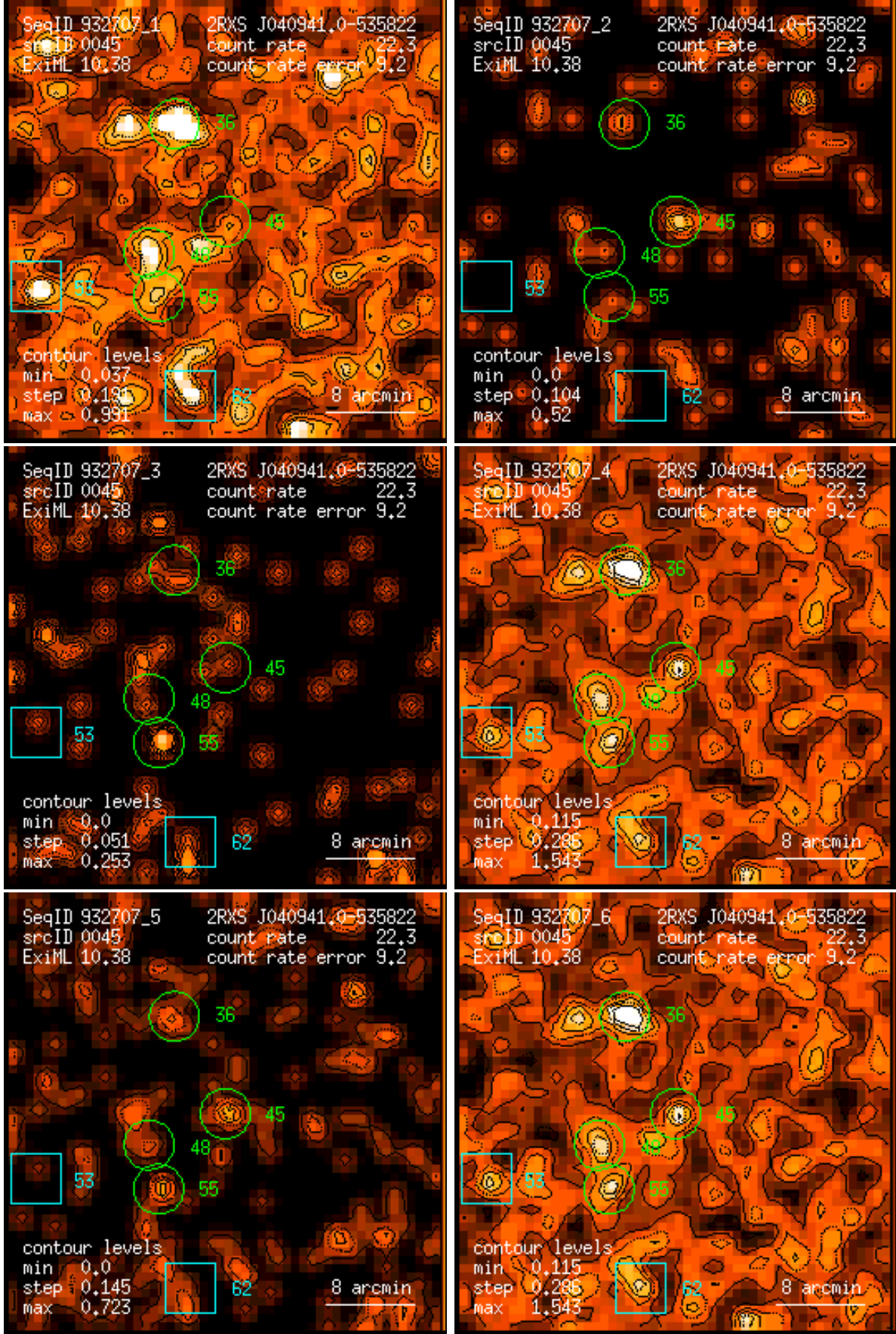
Figure 45: RASS 932707: detection 0045: band rate images, Gaussian filter: (1) PSPC channels 11 – 41, (2) 52 – 90, (3) 91 – 201, (4) 11 – 235, (5) 52 – 201, (6) 11 – 201. Broad band rates in counts/ks. Band rate contour levels in counts/ks/arcmin 2 .
