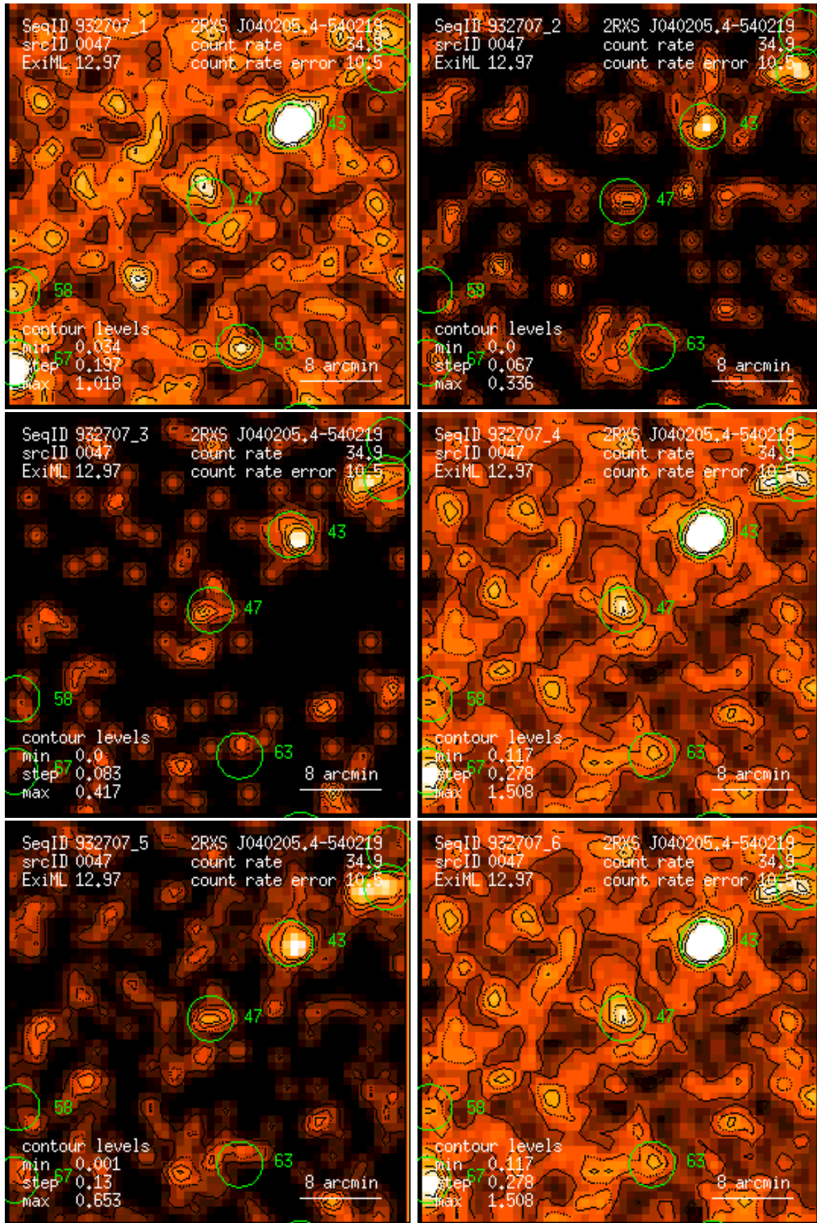
Figure 47: RASS 932707: detection 0047: band rate images, Gaussian filter: (1) PSPC channels 11 – 41, (2) 52 – 90, (3) 91 – 201, (4) 11 – 235, (5) 52 – 201, (6) 11 – 201. Broad band rates in counts/ks. Band rate contour levels in counts/ks/arcmin 2 .
