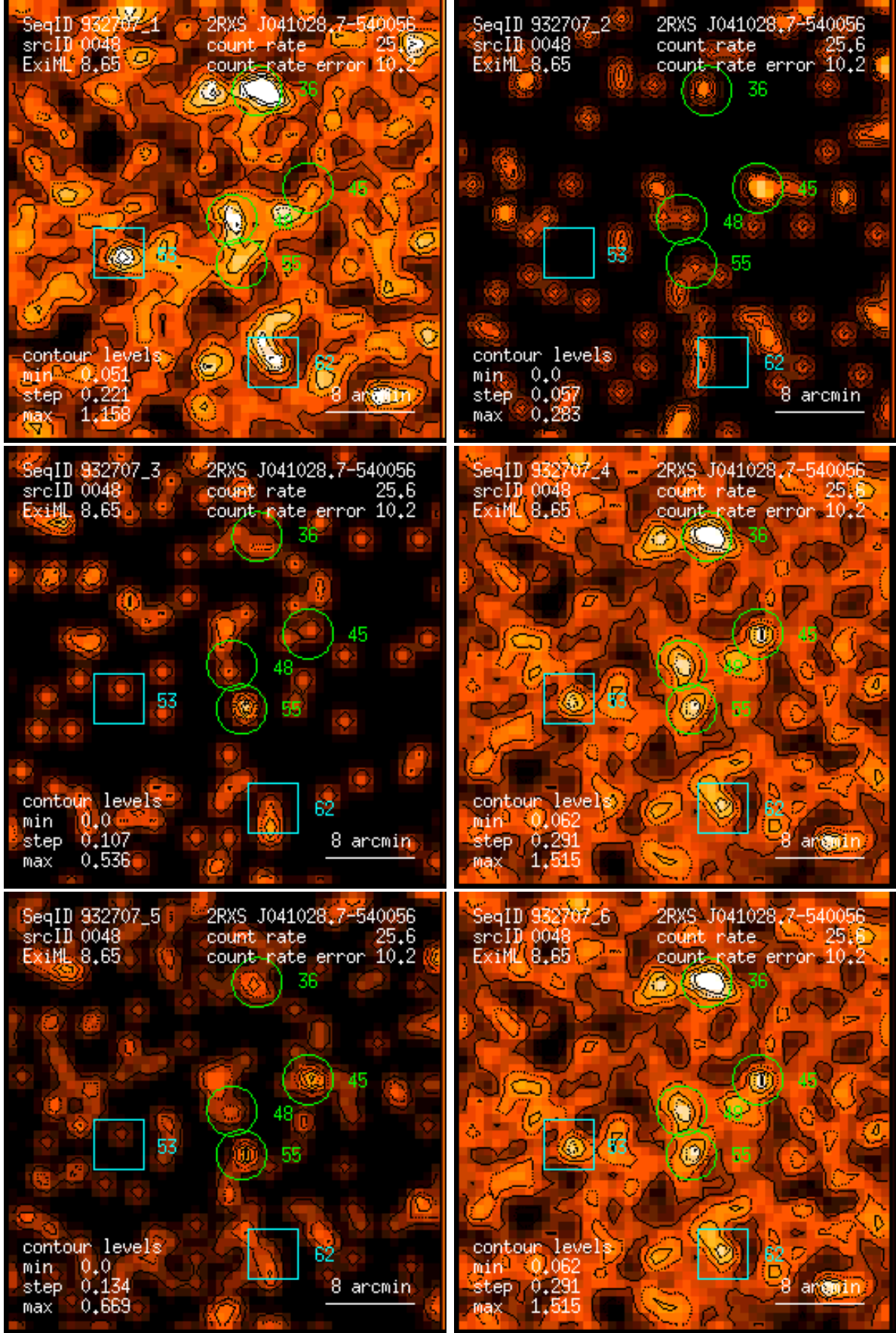
Figure 48: RASS 932707: detection 0048: band rate images, Gaussian filter: (1) PSPC channels 11 – 41, (2) 52 – 90, (3) 91 – 201, (4) 11 – 235, (5) 52 – 201, (6) 11 – 201. Broad band rates in counts/ks. Band rate contour levels in counts/ks/arcmin 2 .
