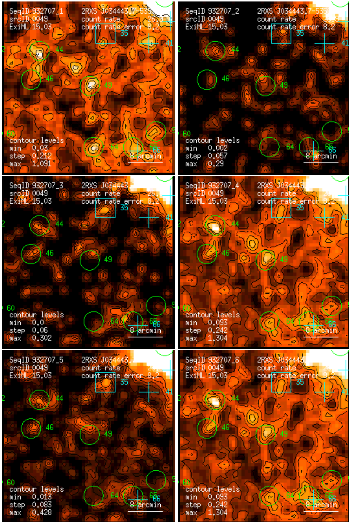
Figure 49: RASS 932707: detection 0049: band rate images, Gaussian filter: (1) PSPC channels 11 – 41, (2) 52 – 90, (3) 91 – 201, (4) 11 – 235, (5) 52 – 201, (6) 11 – 201. Broad band rates in counts/ks. Band rate contour levels in counts/ks/arcmin 2 .
