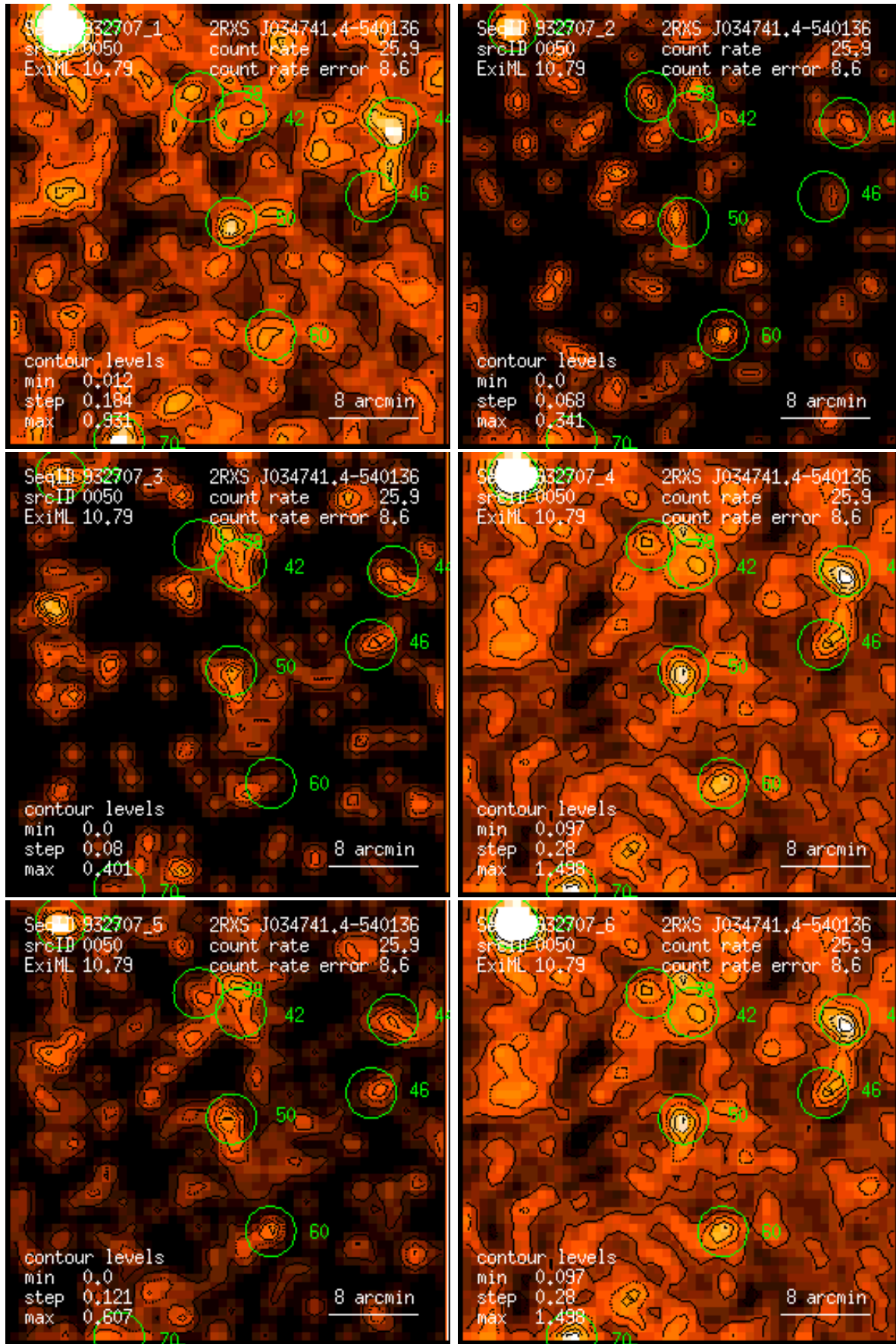
Figure 50: RASS 932707: detection 0050: band rate images, Gaussian filter: (1) PSPC channels 11 – 41, (2) 52 – 90, (3) 91 – 201, (4) 11 – 235, (5) 52 – 201, (6) 11 – 201. Broad band rates in counts/ks. Band rate contour levels in counts/ks/arcmin 2 .
