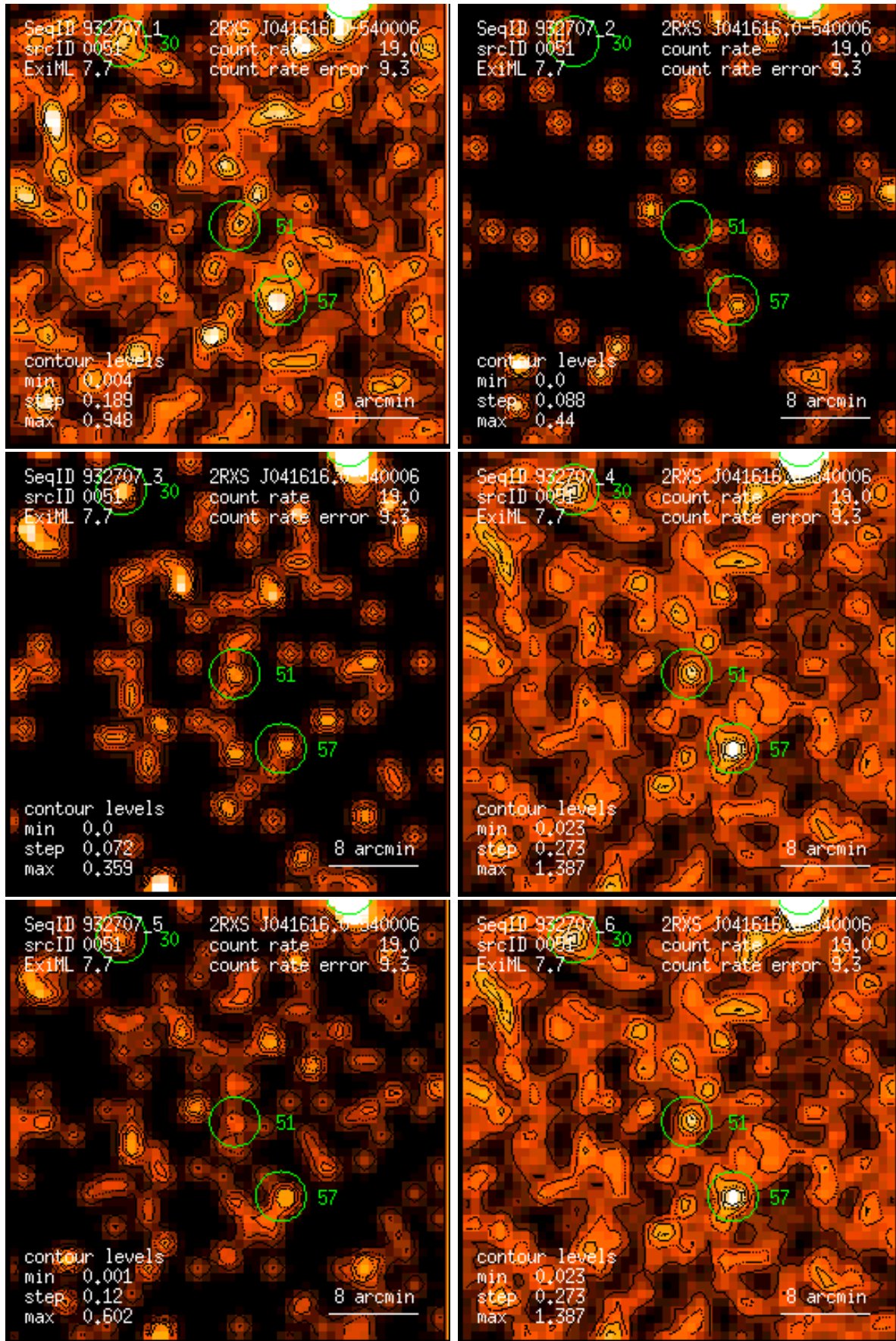
Figure 51: RASS 932707: detection 0051: band rate images, Gaussian filter: (1) PSPC channels 11 – 41, (2) 52 – 90, (3) 91 – 201, (4) 11 – 235, (5) 52 – 201, (6) 11 – 201. Broad band rates in counts/ks. Band rate contour levels in counts/ks/arcmin 2 .
